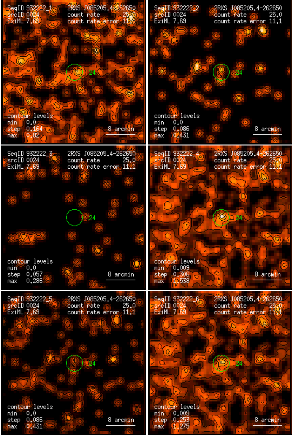
Figure 24: RASS 932222: detection 0024: band rate images, Gaussian filter: (1) PSPC channels 11 – 41, (2) 52 – 90, (3) 91 – 201, (4) 11 – 235, (5) 52 – 201, (6) 11 – 201. Broad band rates in counts/ks. Band rate contour levels in counts/ks/arcmin 2 .
