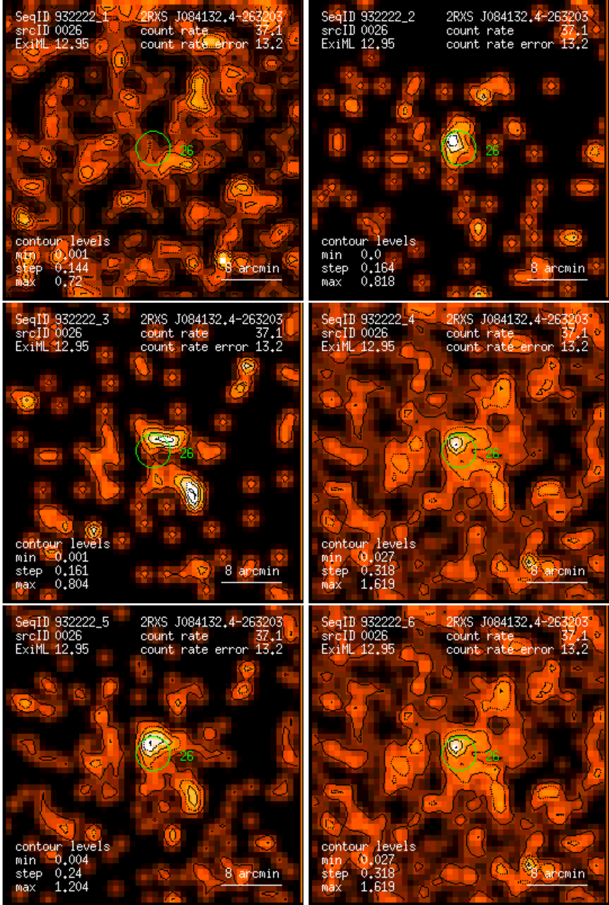
Figure 26: RASS 932222: detection 0026: band rate images, Gaussian filter: (1) PSPC channels 11 – 41, (2) 52 – 90, (3) 91 – 201, (4) 11 – 235, (5) 52 – 201, (6) 11 – 201. Broad band rates in counts/ks. Band rate contour levels in counts/ks/arcmin 2 .
