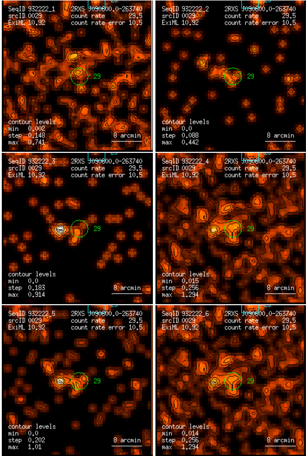
Figure 29: RASS 932222: detection 0029: band rate images, Gaussian filter: (1) PSPC channels 11 – 41, (2) 52 – 90, (3) 91 – 201, (4) 11 – 235, (5) 52 – 201, (6) 11 – 201. Broad band rates in counts/ks. Band rate contour levels in counts/ks/arcmin 2 .
