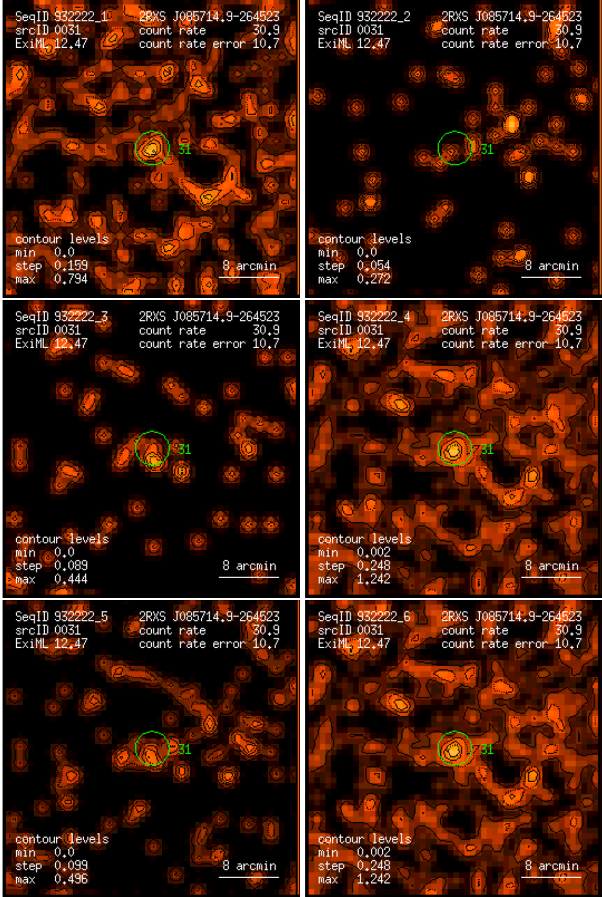
Figure 31: RASS 932222: detection 0031: band rate images, Gaussian filter: (1) PSPC channels 11 – 41, (2) 52 – 90, (3) 91 – 201, (4) 11 – 235, (5) 52 – 201, (6) 11 – 201. Broad band rates in counts/ks. Band rate contour levels in counts/ks/arcmin 2 .
