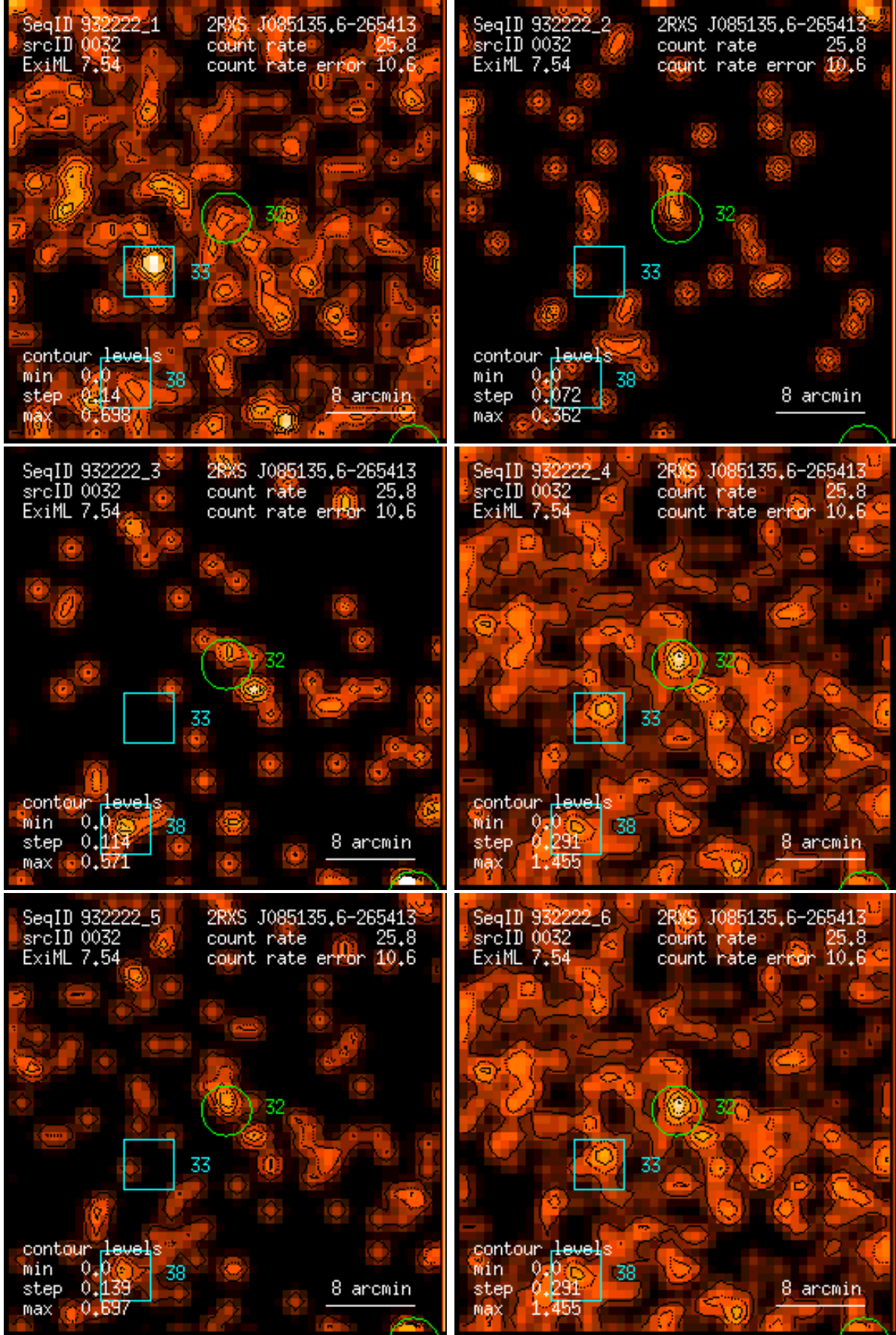
Figure 32: RASS 932222: detection 0032: band rate images, Gaussian filter: (1) PSPC channels 11 – 41, (2) 52 – 90, (3) 91 – 201, (4) 11 – 235, (5) 52 – 201, (6) 11 – 201. Broad band rates in counts/ks. Band rate contour levels in counts/ks/arcmin 2 .
