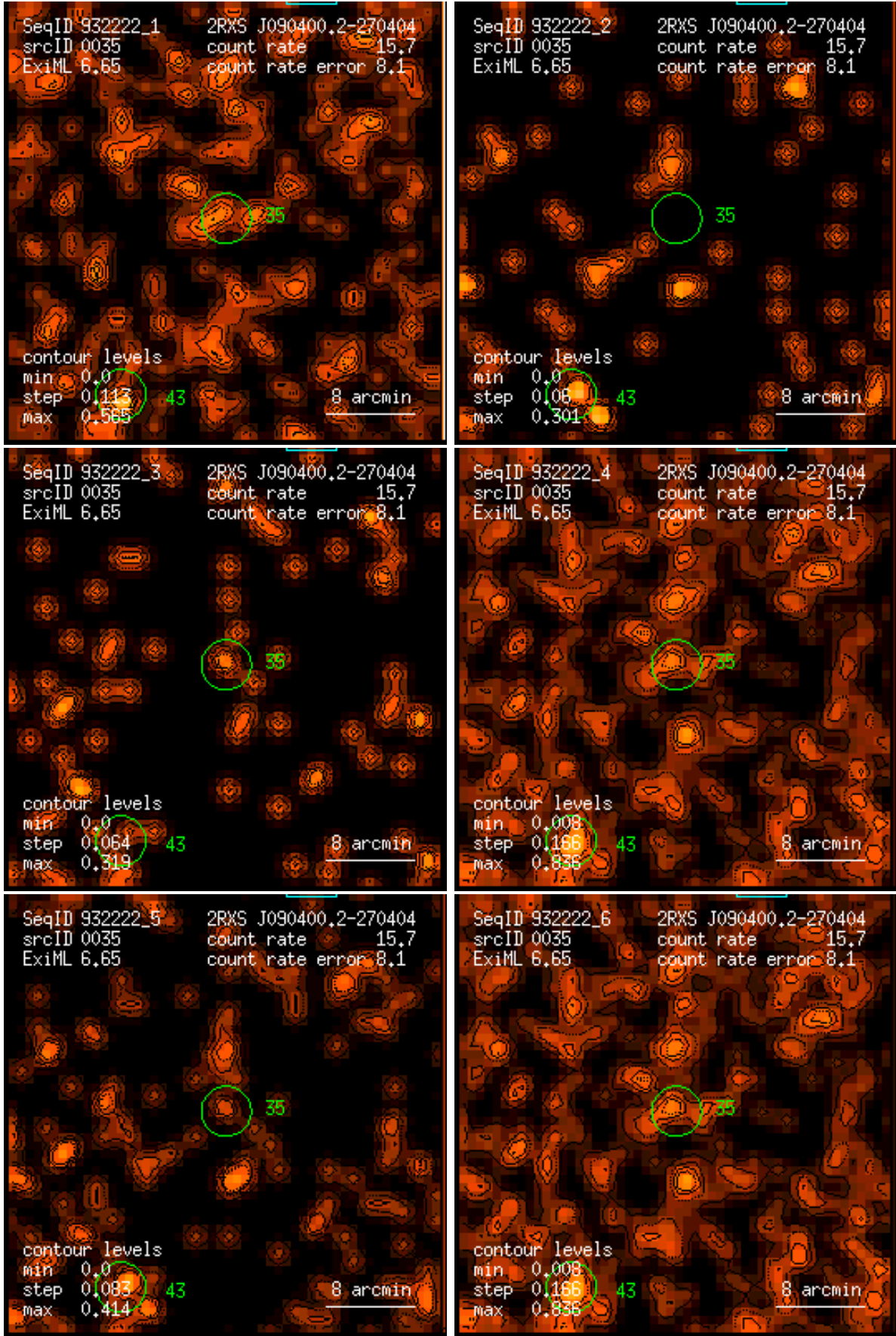
Figure 35: RASS 932222: detection 0035: band rate images, Gaussian filter: (1) PSPC channels 11 – 41, (2) 52 – 90, (3) 91 – 201, (4) 11 – 235, (5) 52 – 201, (6) 11 – 201. Broad band rates in counts/ks. Band rate contour levels in counts/ks/arcmin 2 .
