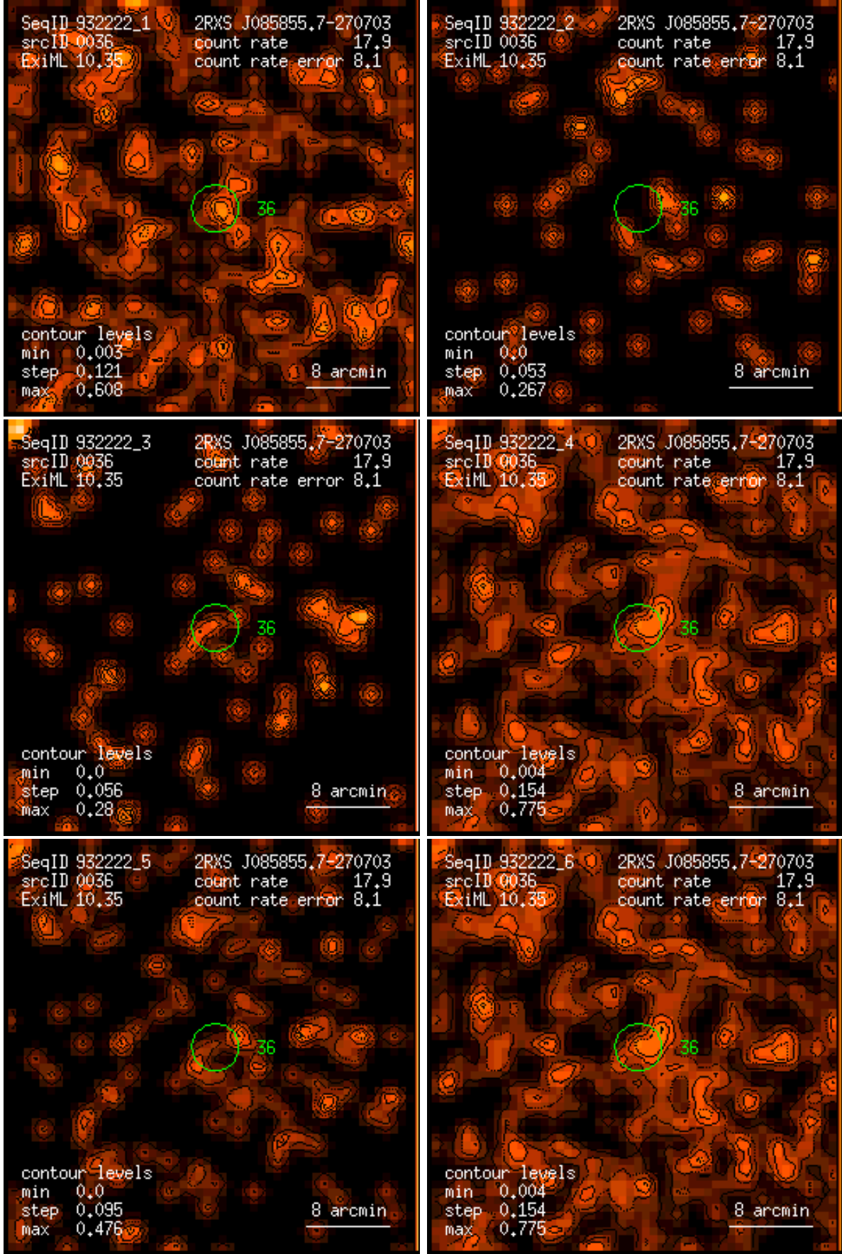
Figure 36: RASS 932222: detection 0036: band rate images, Gaussian filter: (1) PSPC channels 11 – 41, (2) 52 – 90, (3) 91 – 201, (4) 11 – 235, (5) 52 – 201, (6) 11 – 201. Broad band rates in counts/ks. Band rate contour levels in counts/ks/arcmin 2 .
