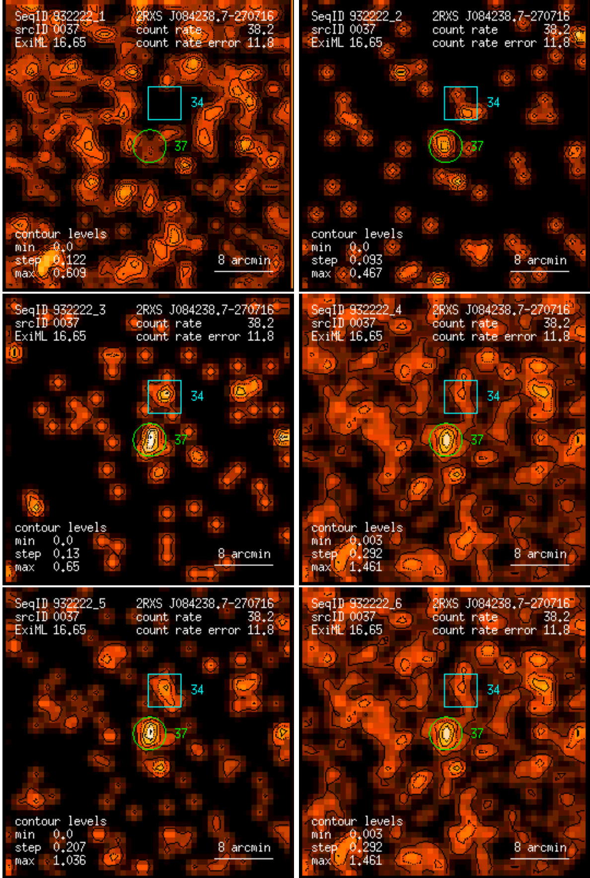
Figure 37: RASS 932222: detection 0037: band rate images, Gaussian filter: (1) PSPC channels 11 – 41, (2) 52 – 90, (3) 91 – 201, (4) 11 – 235, (5) 52 – 201, (6) 11 – 201. Broad band rates in counts/ks. Band rate contour levels in counts/ks/arcmin 2 .
