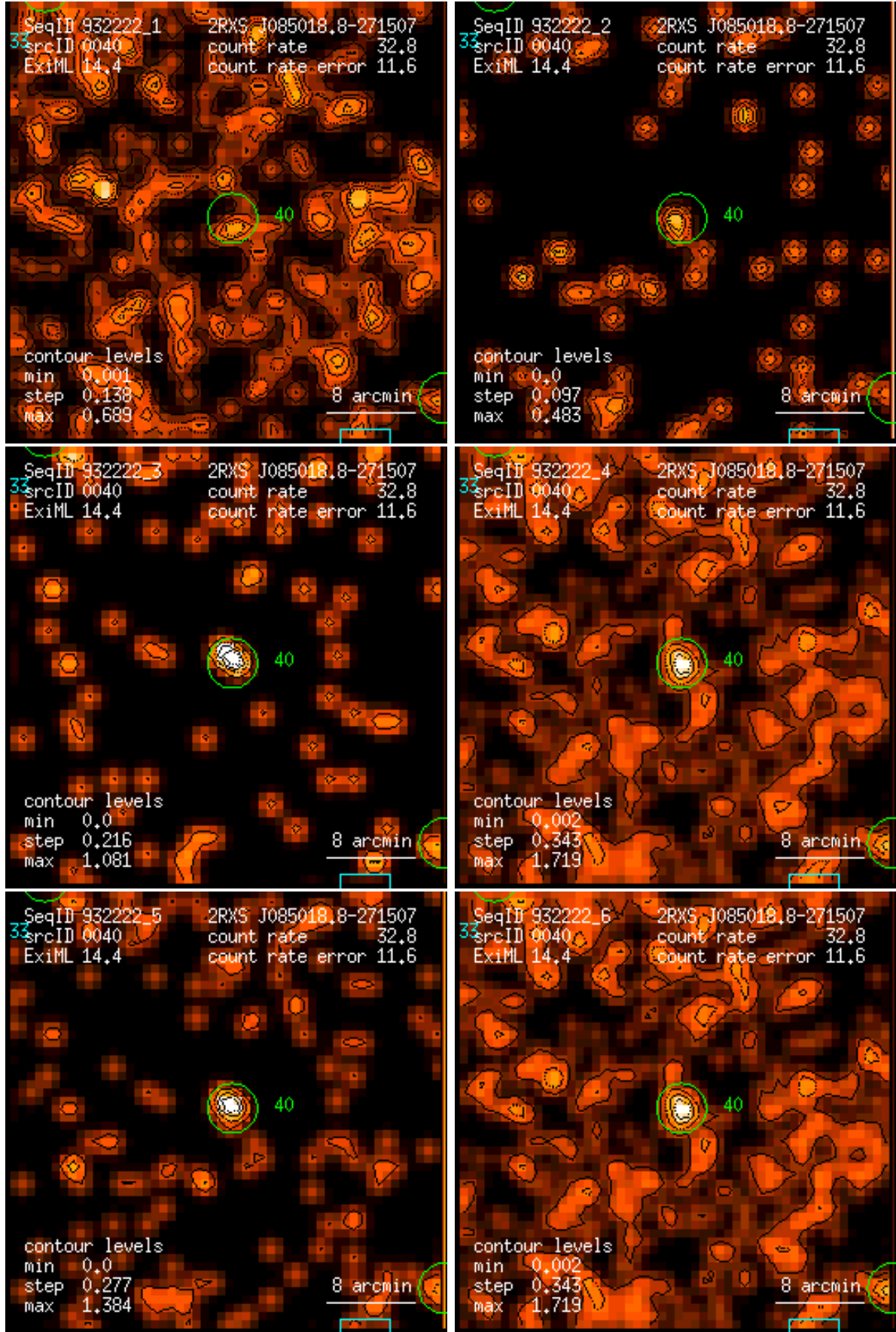
Figure 40: RASS 932222: detection 0040: band rate images, Gaussian filter: (1) PSPC channels 11 – 41, (2) 52 – 90, (3) 91 – 201, (4) 11 – 235, (5) 52 – 201, (6) 11 – 201. Broad band rates in counts/ks. Band rate contour levels in counts/ks/arcmin 2 .
