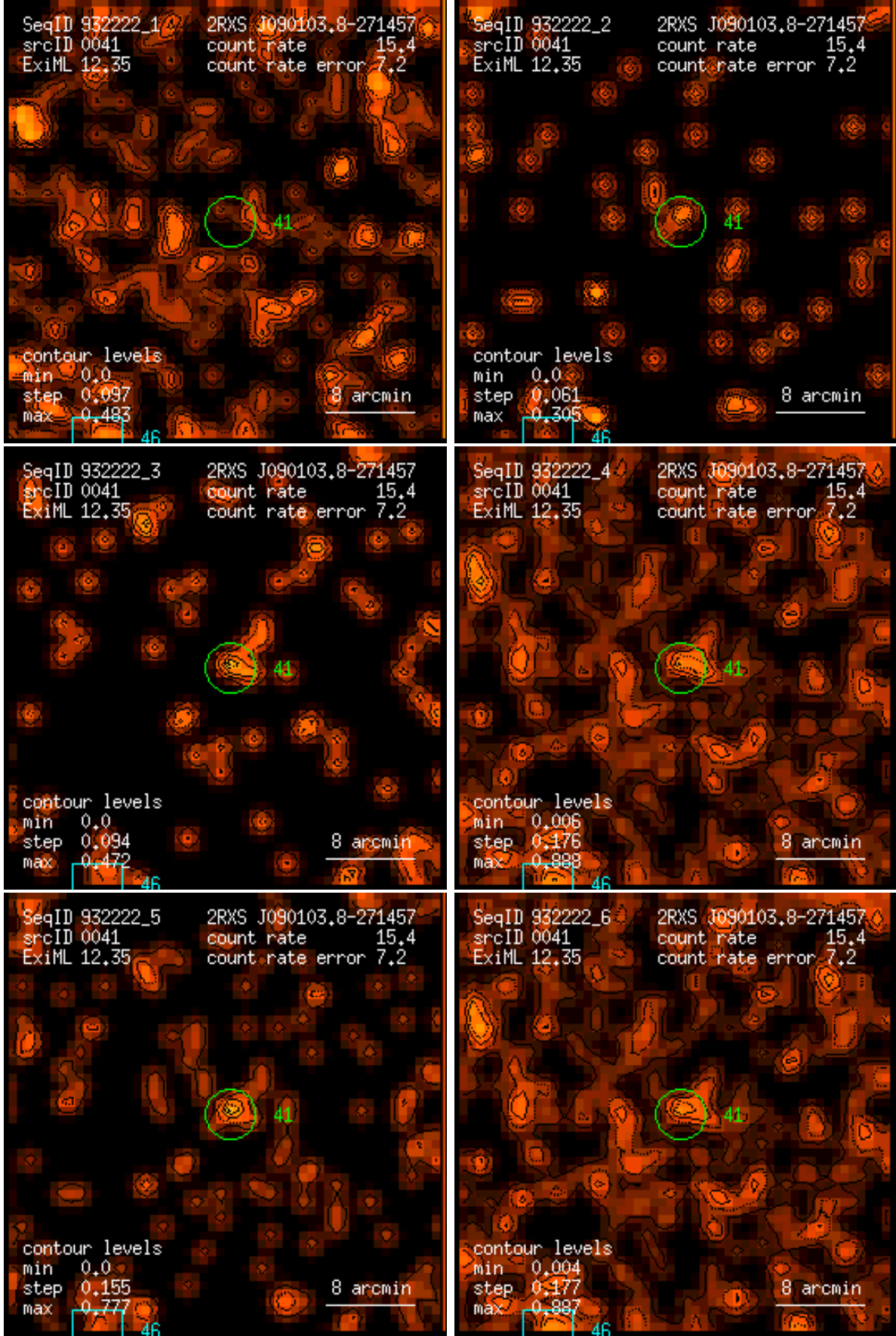
Figure 41: RASS 932222: detection 0041: band rate images, Gaussian filter: (1) PSPC channels 11 – 41, (2) 52 – 90, (3) 91 – 201, (4) 11 – 235, (5) 52 – 201, (6) 11 – 201. Broad band rates in counts/ks. Band rate contour levels in counts/ks/arcmin 2 .
