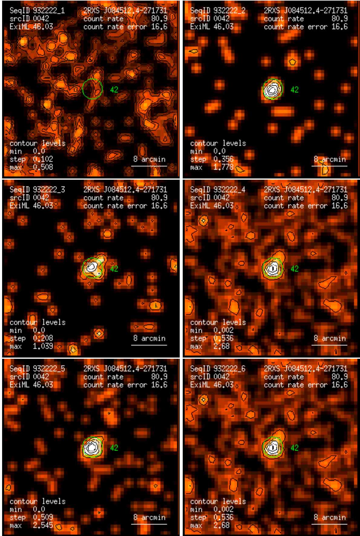
Figure 42: RASS 932222: detection 0042: band rate images, Gaussian filter: (1) PSPC channels 11 – 41, (2) 52 – 90, (3) 91 – 201, (4) 11 – 235, (5) 52 – 201, (6) 11 – 201. Broad band rates in counts/ks. Band rate contour levels in counts/ks/arcmin 2 .
