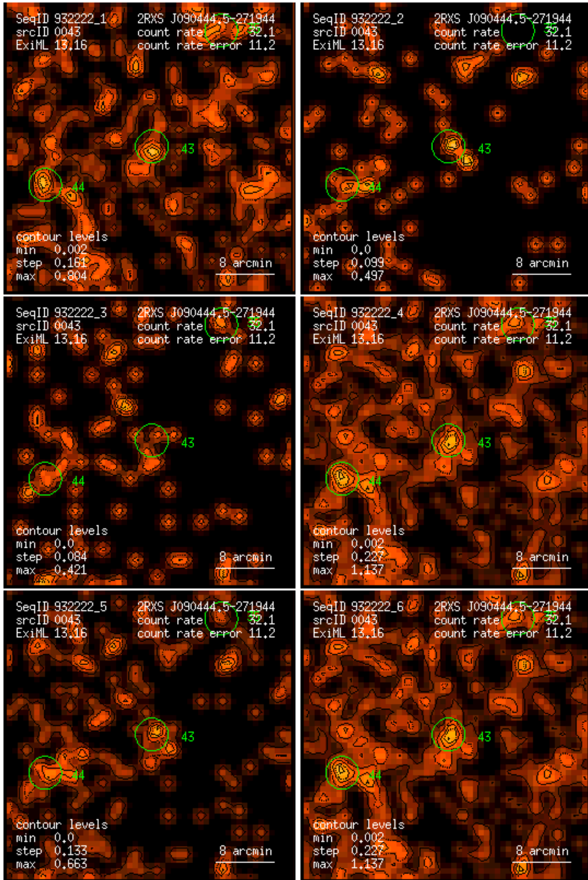
Figure 43: RASS 932222: detection 0043: band rate images, Gaussian filter: (1) PSPC channels 11 – 41, (2) 52 – 90, (3) 91 – 201, (4) 11 – 235, (5) 52 – 201, (6) 11 – 201. Broad band rates in counts/ks. Band rate contour levels in counts/ks/arcmin 2 .
