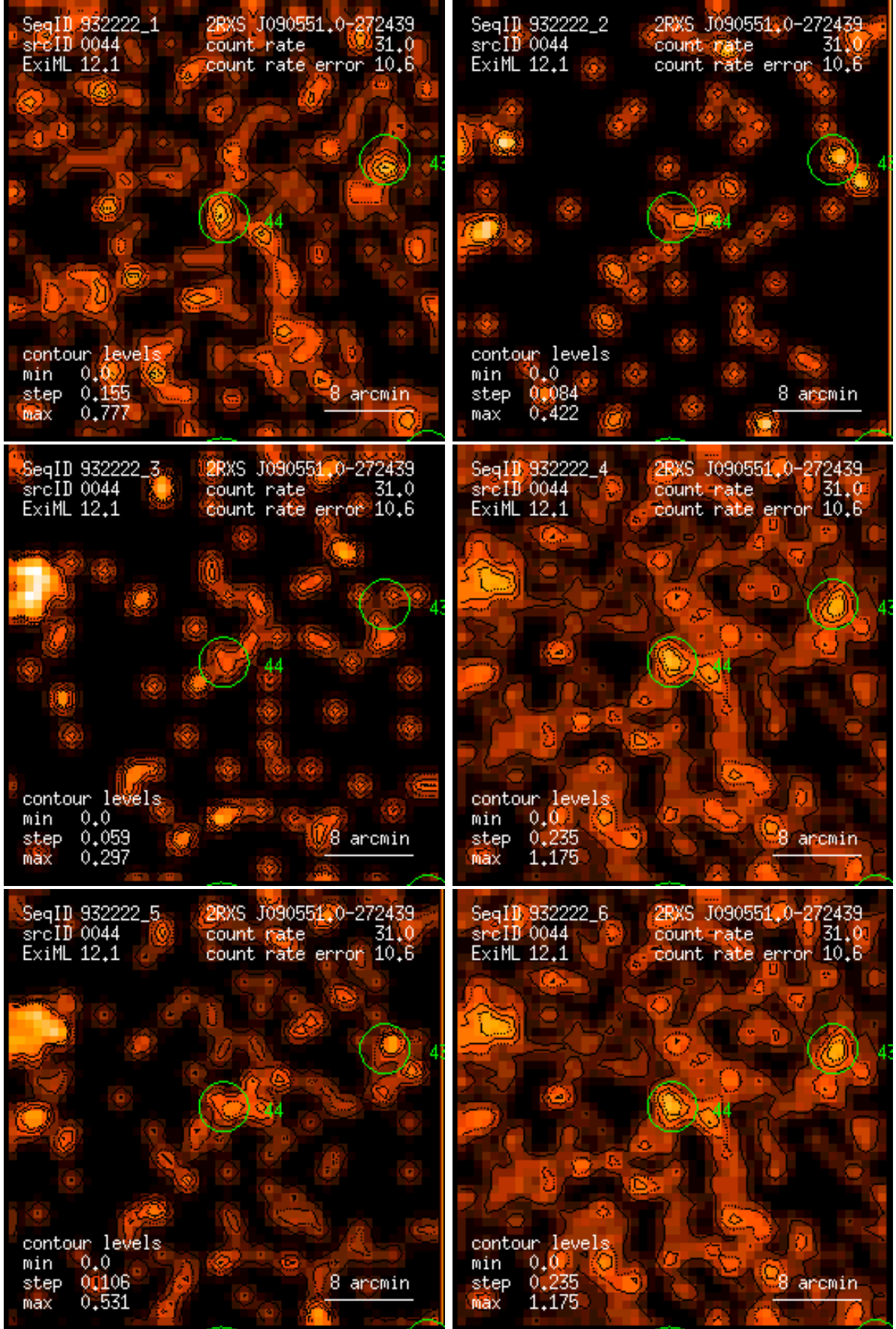
Figure 44: RASS 932222: detection 0044: band rate images, Gaussian filter: (1) PSPC channels 11 – 41, (2) 52 – 90, (3) 91 – 201, (4) 11 – 235, (5) 52 – 201, (6) 11 – 201. Broad band rates in counts/ks. Band rate contour levels in counts/ks/arcmin 2 .
