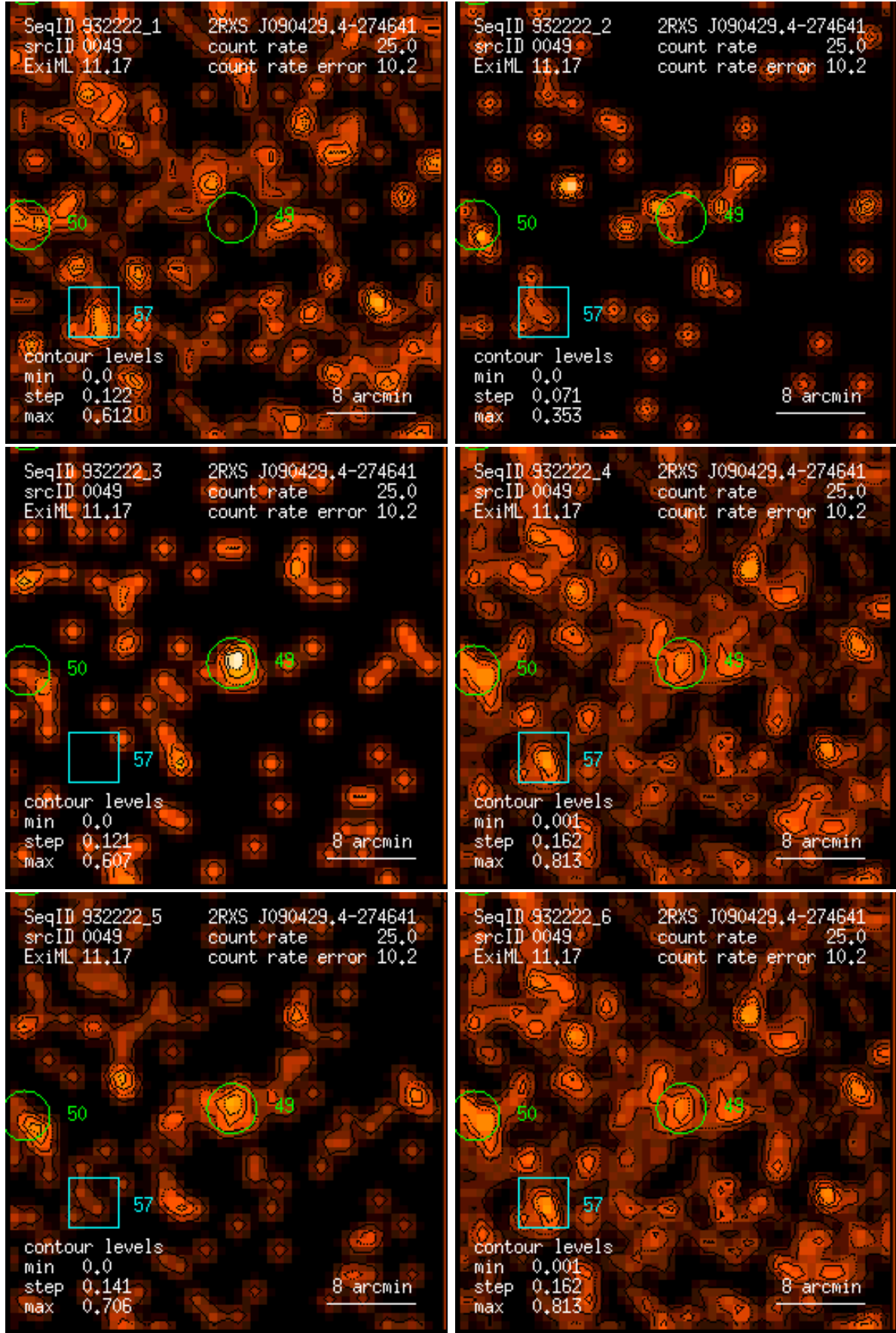
Figure 49: RASS 932222: detection 0049: band rate images, Gaussian filter: (1) PSPC channels 11 – 41, (2) 52 – 90, (3) 91 – 201, (4) 11 – 235, (5) 52 – 201, (6) 11 – 201. Broad band rates in counts/ks. Band rate contour levels in counts/ks/arcmin 2 .
