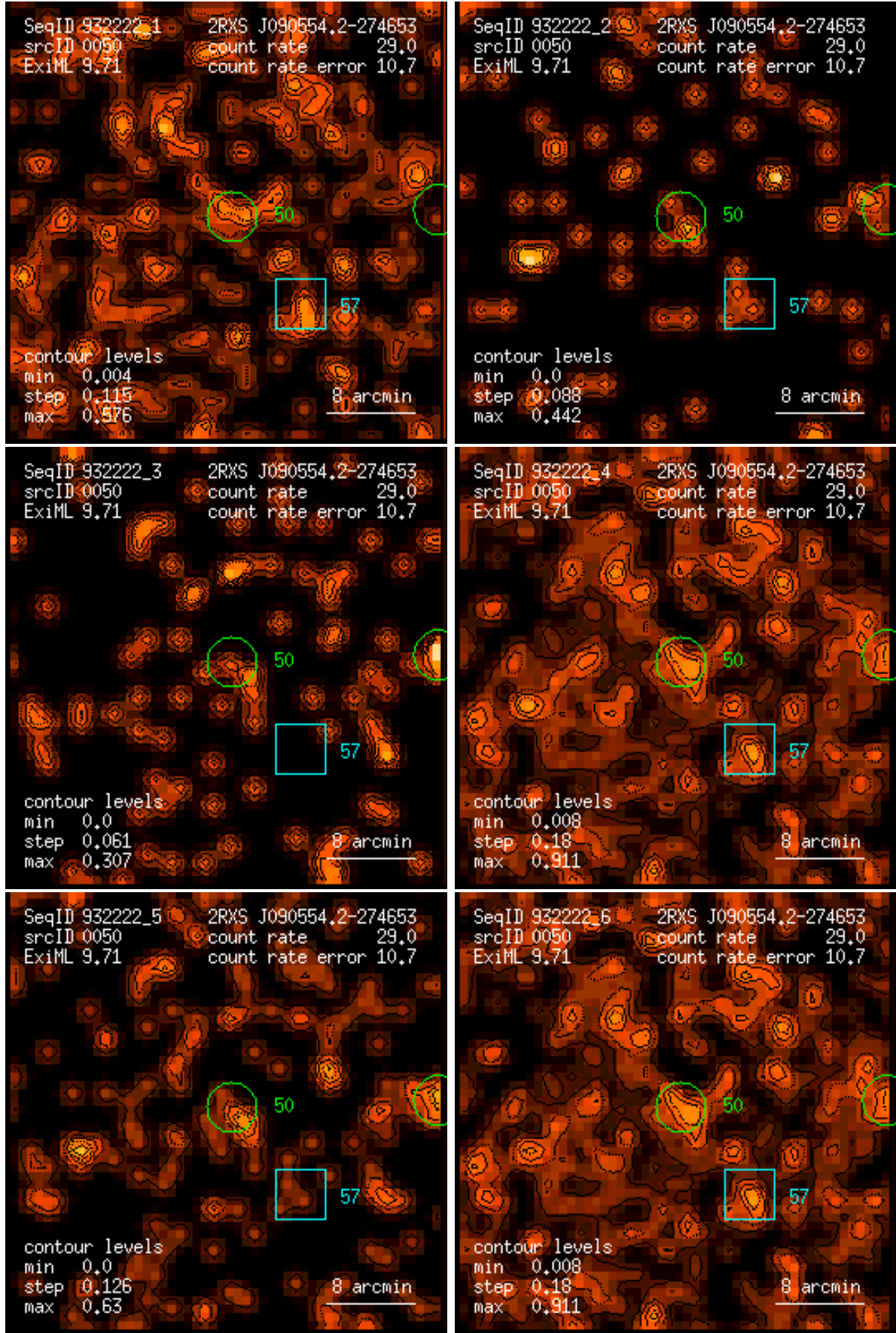
Figure 50: RASS 932222: detection 0050: band rate images, Gaussian filter: (1) PSPC channels 11 – 41, (2) 52 – 90, (3) 91 – 201, (4) 11 – 235, (5) 52 – 201, (6) 11 – 201. Broad band rates in counts/ks. Band rate contour levels in counts/ks/arcmin 2 .
