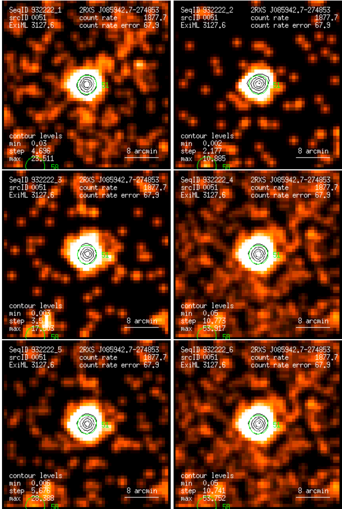
Figure 51: RASS 932222: detection 0051: band rate images, Gaussian filter: (1) PSPC channels 11 – 41, (2) 52 – 90, (3) 91 – 201, (4) 11 – 235, (5) 52 – 201, (6) 11 – 201. Broad band rates in counts/ks. Band rate contour levels in counts/ks/arcmin 2 .
