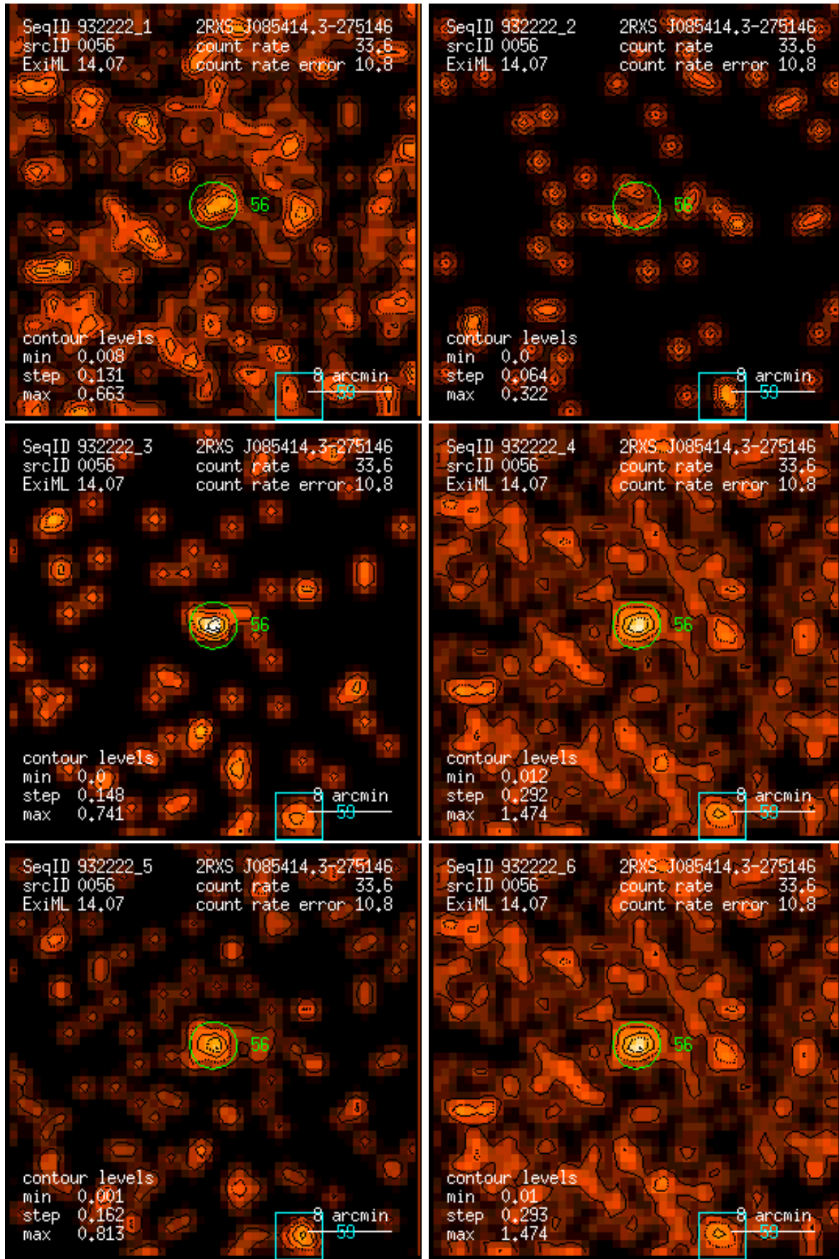
Figure 56: RASS 932222: detection 0056: band rate images, Gaussian filter: (1) PSPC channels 11 – 41, (2) 52 – 90, (3) 91 – 201, (4) 11 – 235, (5) 52 – 201, (6) 11 – 201. Broad band rates in counts/ks. Band rate contour levels in counts/ks/arcmin 2 .
