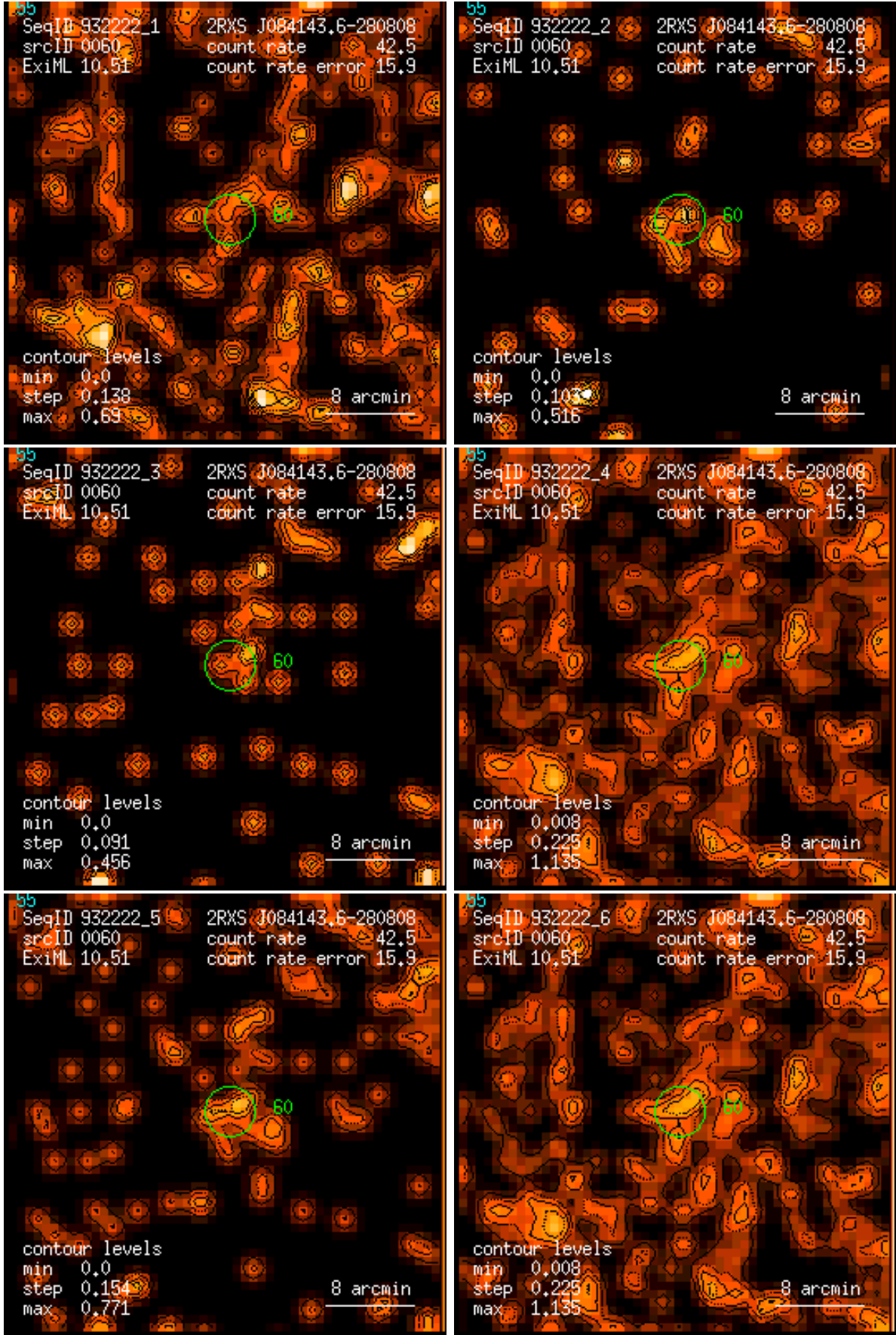
Figure 60: RASS 932222: detection 0060: band rate images, Gaussian filter: (1) PSPC channels 11 – 41, (2) 52 – 90, (3) 91 – 201, (4) 11 – 235, (5) 52 – 201, (6) 11 – 201. Broad band rates in counts/ks. Band rate contour levels in counts/ks/arcmin 2 .
