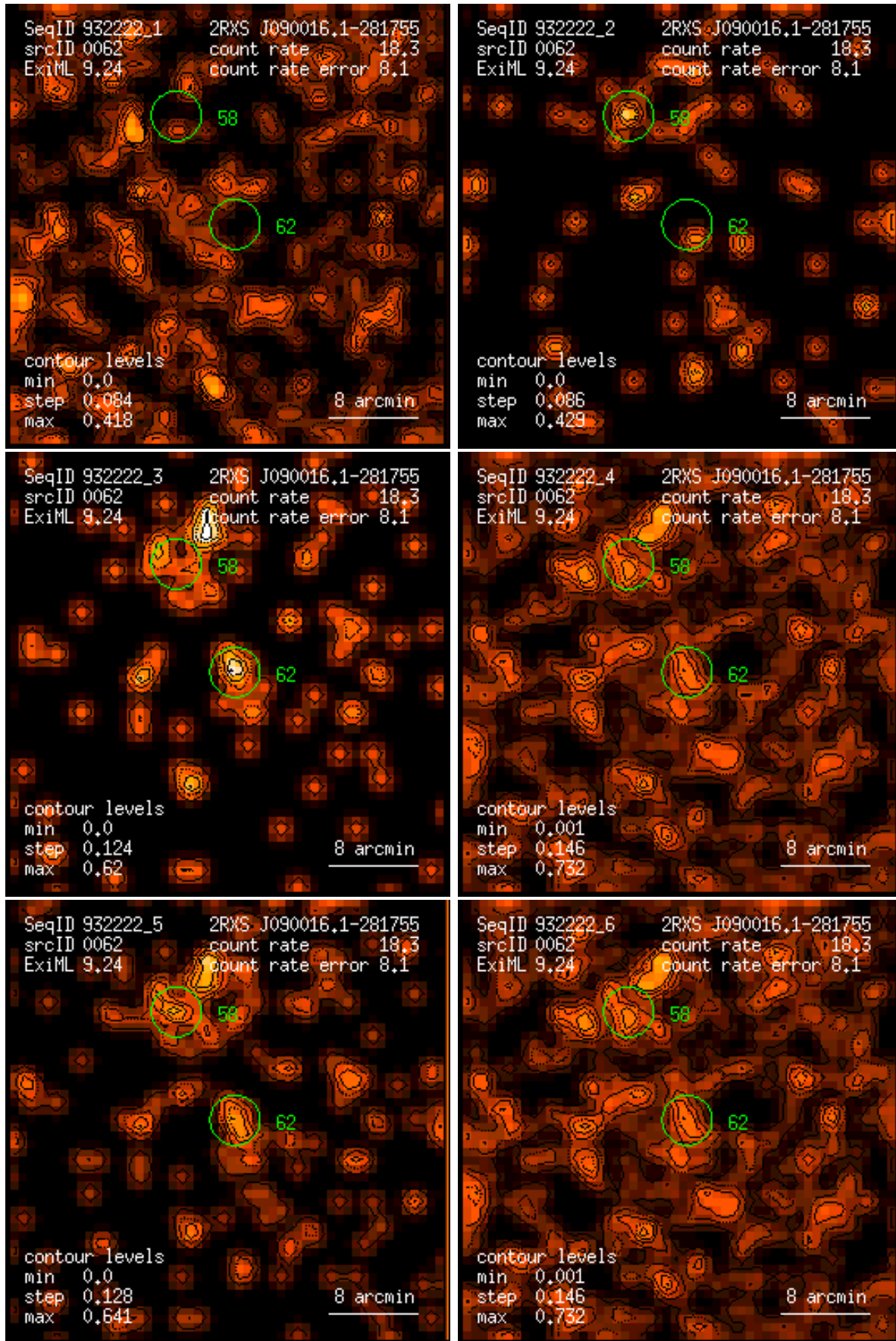
Figure 62: RASS 932222: detection 0062: band rate images, Gaussian filter: (1) PSPC channels 11 – 41, (2) 52 – 90, (3) 91 – 201, (4) 11 – 235, (5) 52 – 201, (6) 11 – 201. Broad band rates in counts/ks. Band rate contour levels in counts/ks/arcmin 2 .
