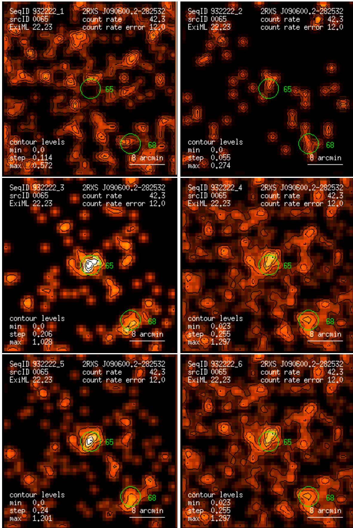
Figure 65: RASS 932222: detection 0065: band rate images, Gaussian filter: (1) PSPC channels 11 – 41, (2) 52 – 90, (3) 91 – 201, (4) 11 – 235, (5) 52 – 201, (6) 11 – 201. Broad band rates in counts/ks. Band rate contour levels in counts/ks/arcmin 2 .
