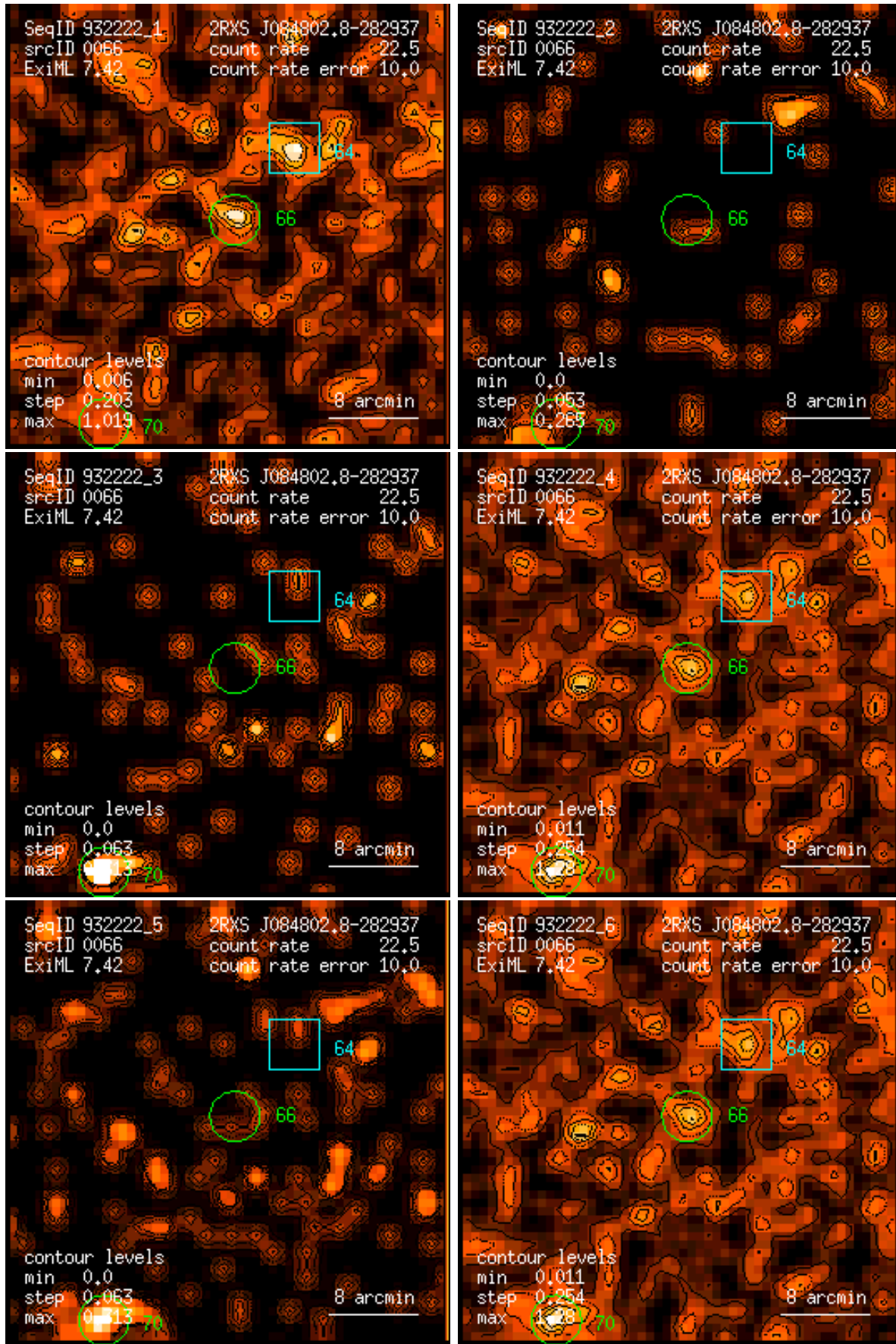
Figure 66: RASS 932222: detection 0066: band rate images, Gaussian filter: (1) PSPC channels 11 – 41, (2) 52 – 90, (3) 91 – 201, (4) 11 – 235, (5) 52 – 201, (6) 11 – 201. Broad band rates in counts/ks. Band rate contour levels in counts/ks/arcmin 2 .
