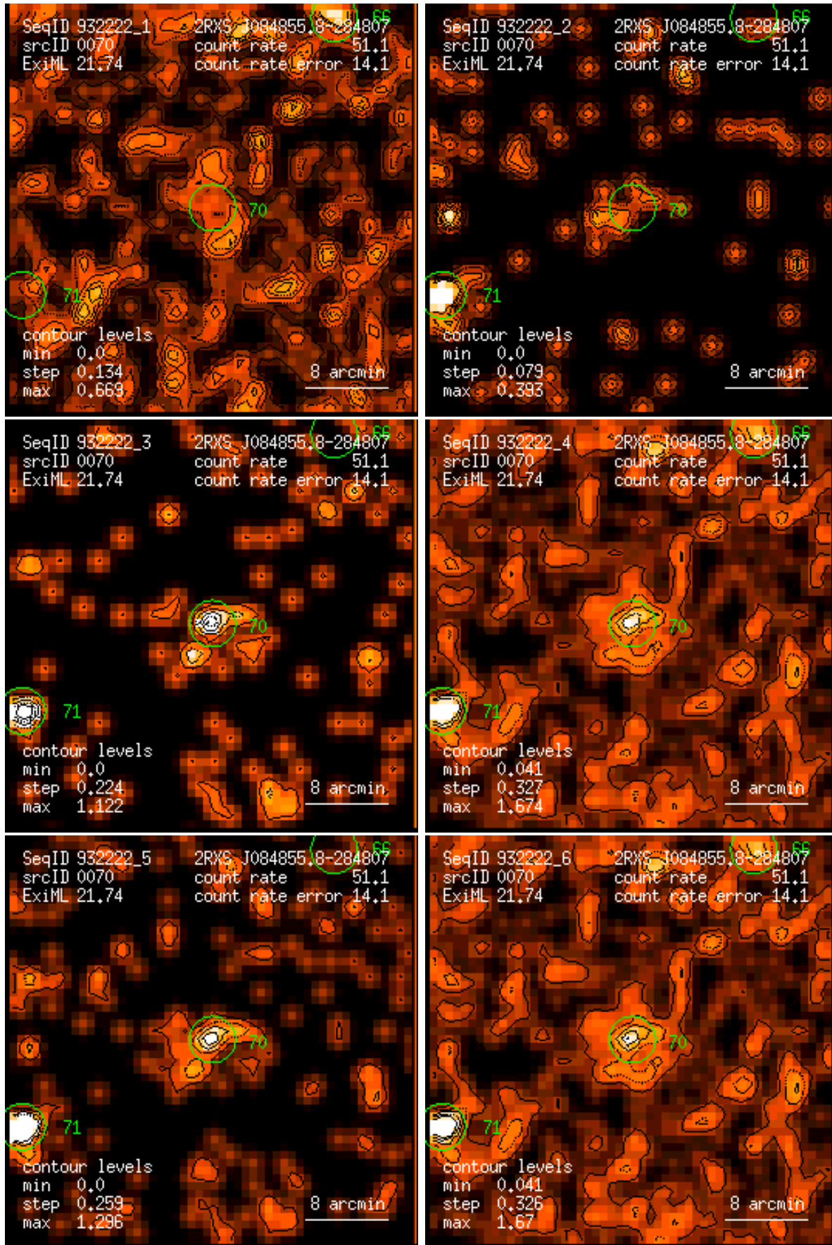
Figure 70: RASS 932222: detection 0070: band rate images, Gaussian filter: (1) PSPC channels 11 – 41, (2) 52 – 90, (3) 91 – 201, (4) 11 – 235, (5) 52 – 201, (6) 11 – 201. Broad band rates in counts/ks. Band rate contour levels in counts/ks/arcmin 2 .
