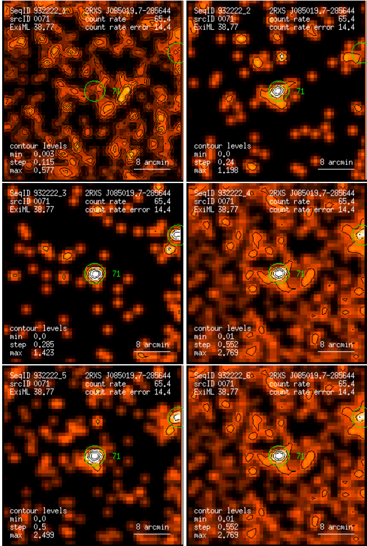
Figure 71: RASS 932222: detection 0071: band rate images, Gaussian filter: (1) PSPC channels 11 – 41, (2) 52 – 90, (3) 91 – 201, (4) 11 – 235, (5) 52 – 201, (6) 11 – 201. Broad band rates in counts/ks. Band rate contour levels in counts/ks/arcmin 2 .
