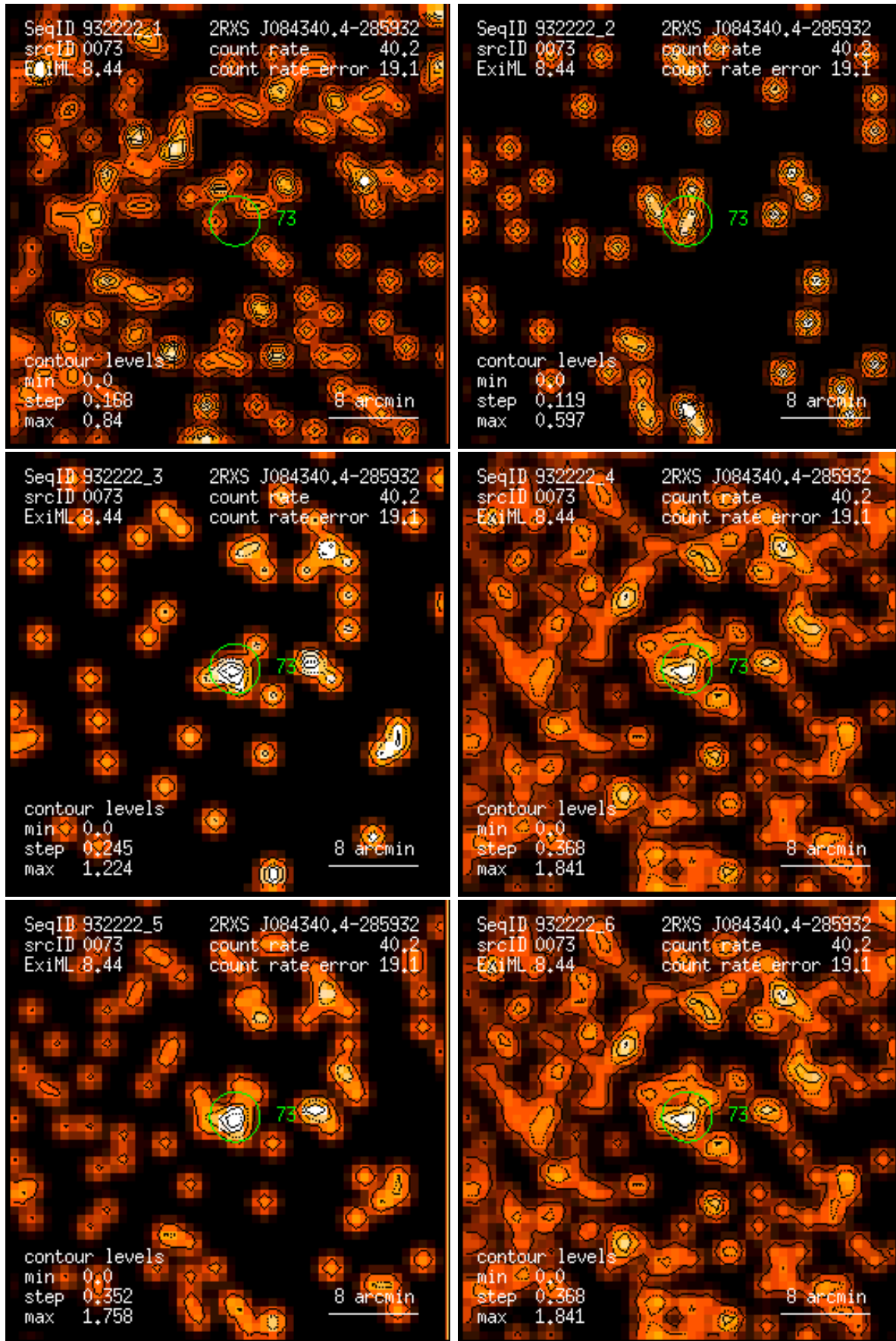
Figure 73: RASS 932222: detection 0073: band rate images, Gaussian filter: (1) PSPC channels 11 – 41, (2) 52 – 90, (3) 91 – 201, (4) 11 – 235, (5) 52 – 201, (6) 11 – 201. Broad band rates in counts/ks. Band rate contour levels in counts/ks/arcmin 2 .
