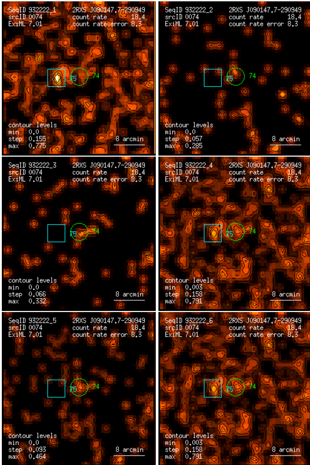
Figure 74: RASS 932222: detection 0074: band rate images, Gaussian filter: (1) PSPC channels 11 – 41, (2) 52 – 90, (3) 91 – 201, (4) 11 – 235, (5) 52 – 201, (6) 11 – 201. Broad band rates in counts/ks. Band rate contour levels in counts/ks/arcmin 2 .
