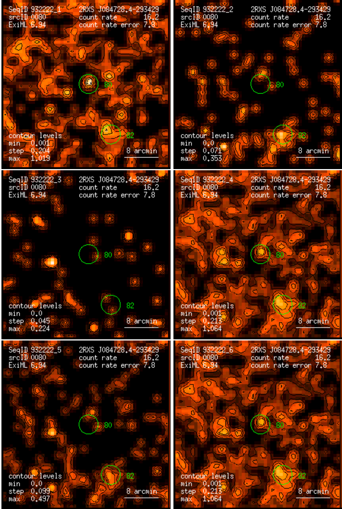
Figure 80: RASS 932222: detection 0080: band rate images, Gaussian filter: (1) PSPC channels 11 – 41, (2) 52 – 90, (3) 91 – 201, (4) 11 – 235, (5) 52 – 201, (6) 11 – 201. Broad band rates in counts/ks. Band rate contour levels in counts/ks/arcmin 2 .
