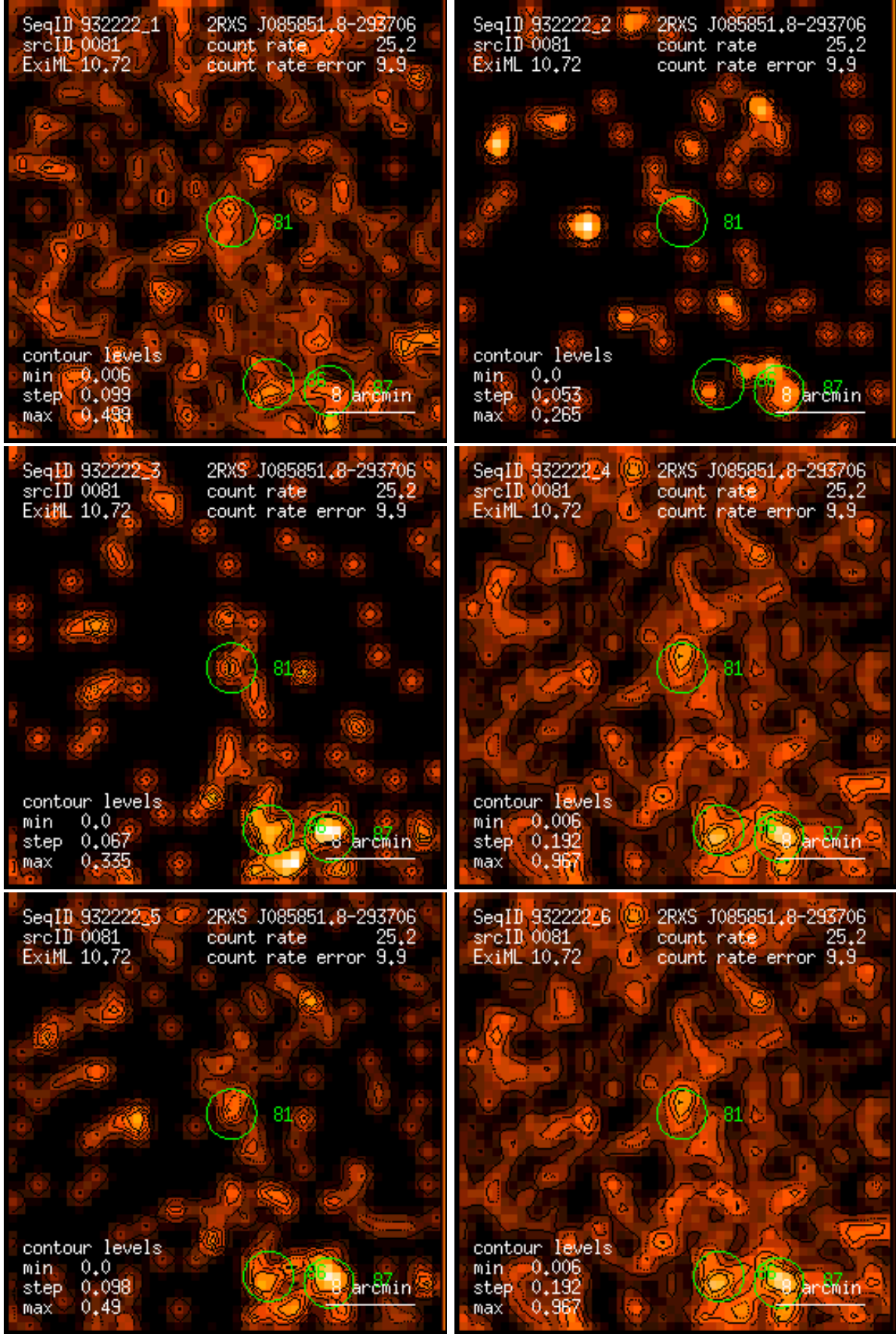
Figure 81: RASS 932222: detection 0081: band rate images, Gaussian filter: (1) PSPC channels 11 – 41, (2) 52 – 90, (3) 91 – 201, (4) 11 – 235, (5) 52 – 201, (6) 11 – 201. Broad band rates in counts/ks. Band rate contour levels in counts/ks/arcmin 2 .
