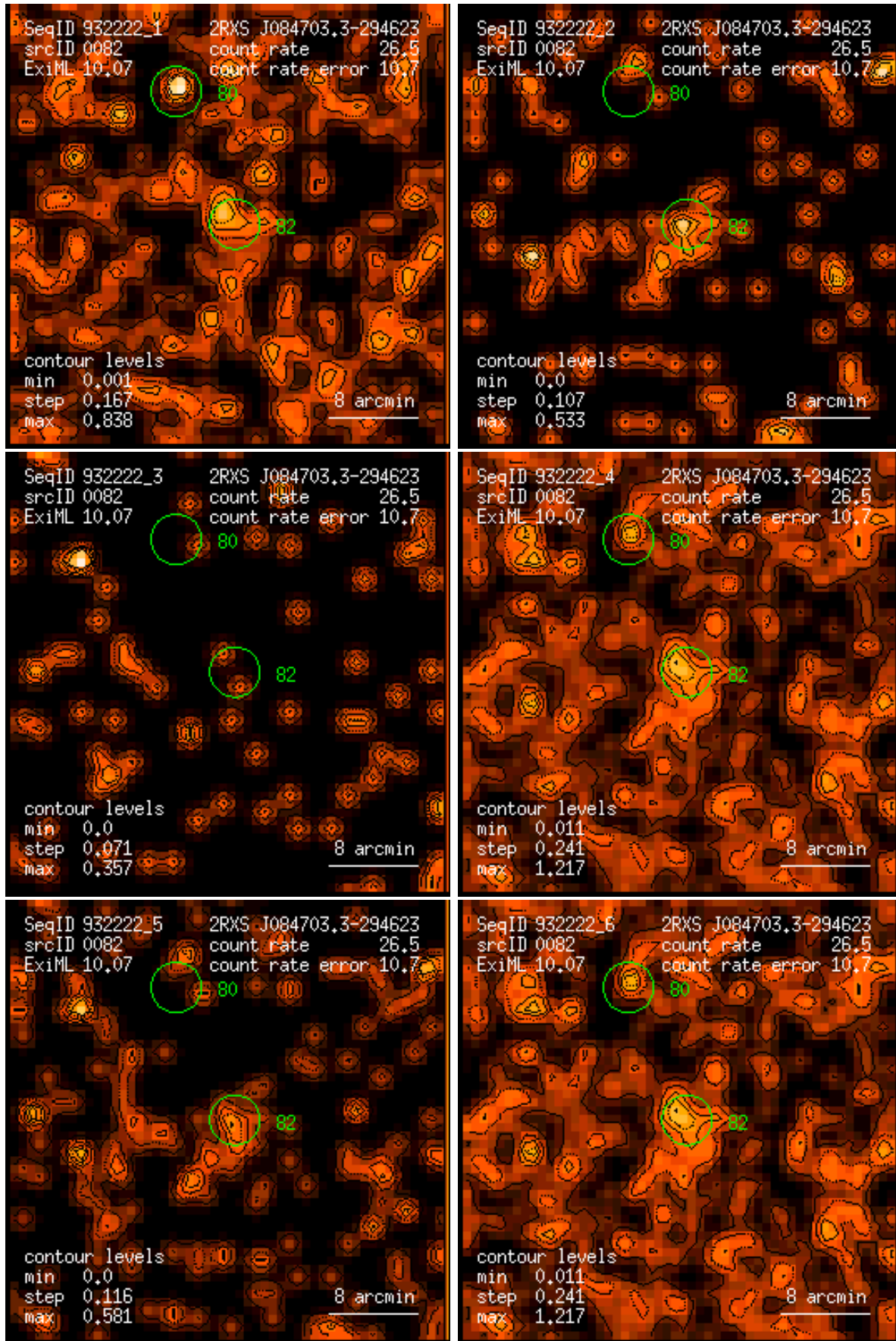
Figure 82: RASS 932222: detection 0082: band rate images, Gaussian filter: (1) PSPC channels 11 – 41, (2) 52 – 90, (3) 91 – 201, (4) 11 – 235, (5) 52 – 201, (6) 11 – 201. Broad band rates in counts/ks. Band rate contour levels in counts/ks/arcmin 2 .
