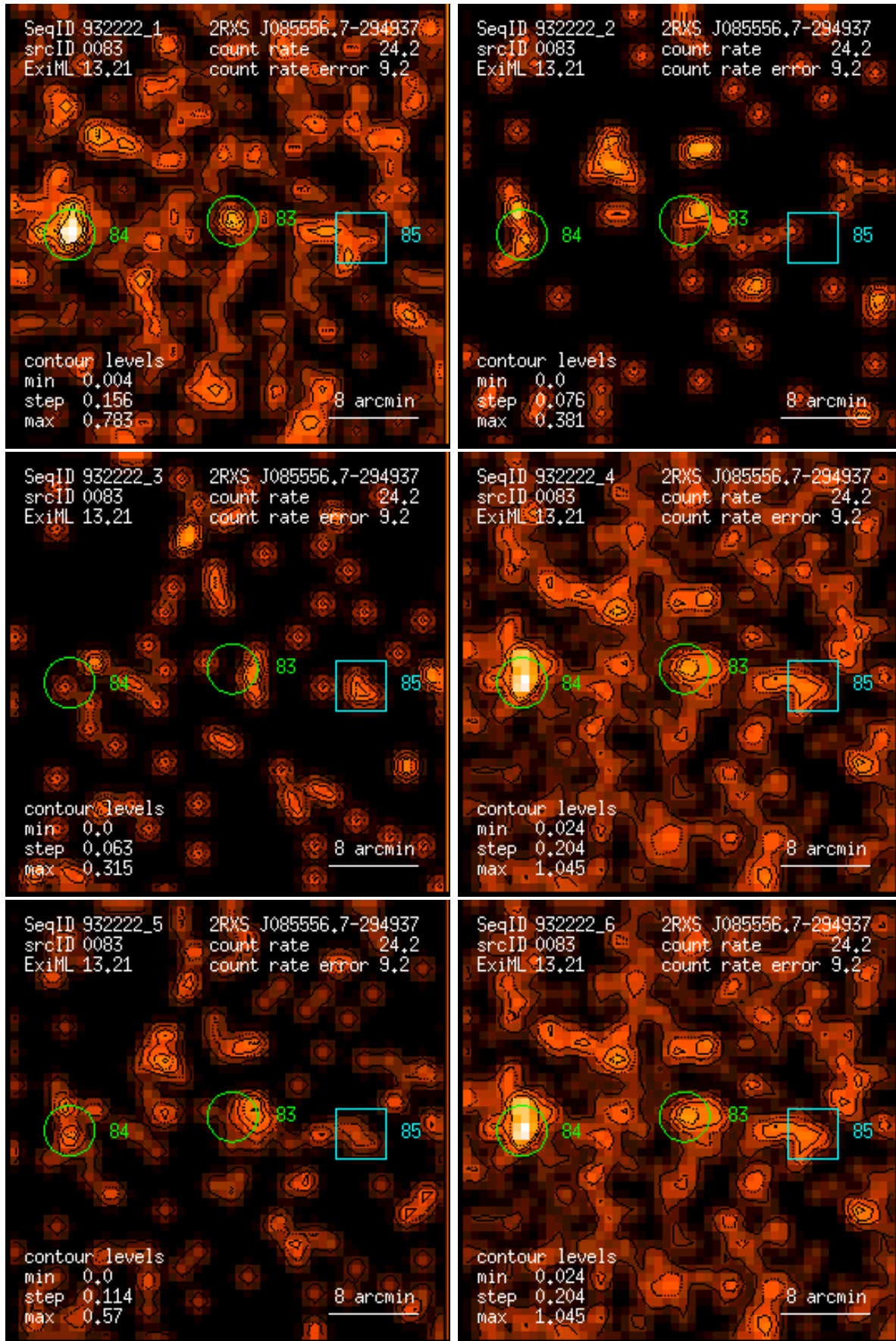
Figure 83: RASS 932222: detection 0083: band rate images, Gaussian filter: (1) PSPC channels 11 – 41, (2) 52 – 90, (3) 91 – 201, (4) 11 – 235, (5) 52 – 201, (6) 11 – 201. Broad band rates in counts/ks. Band rate contour levels in counts/ks/arcmin 2 .
