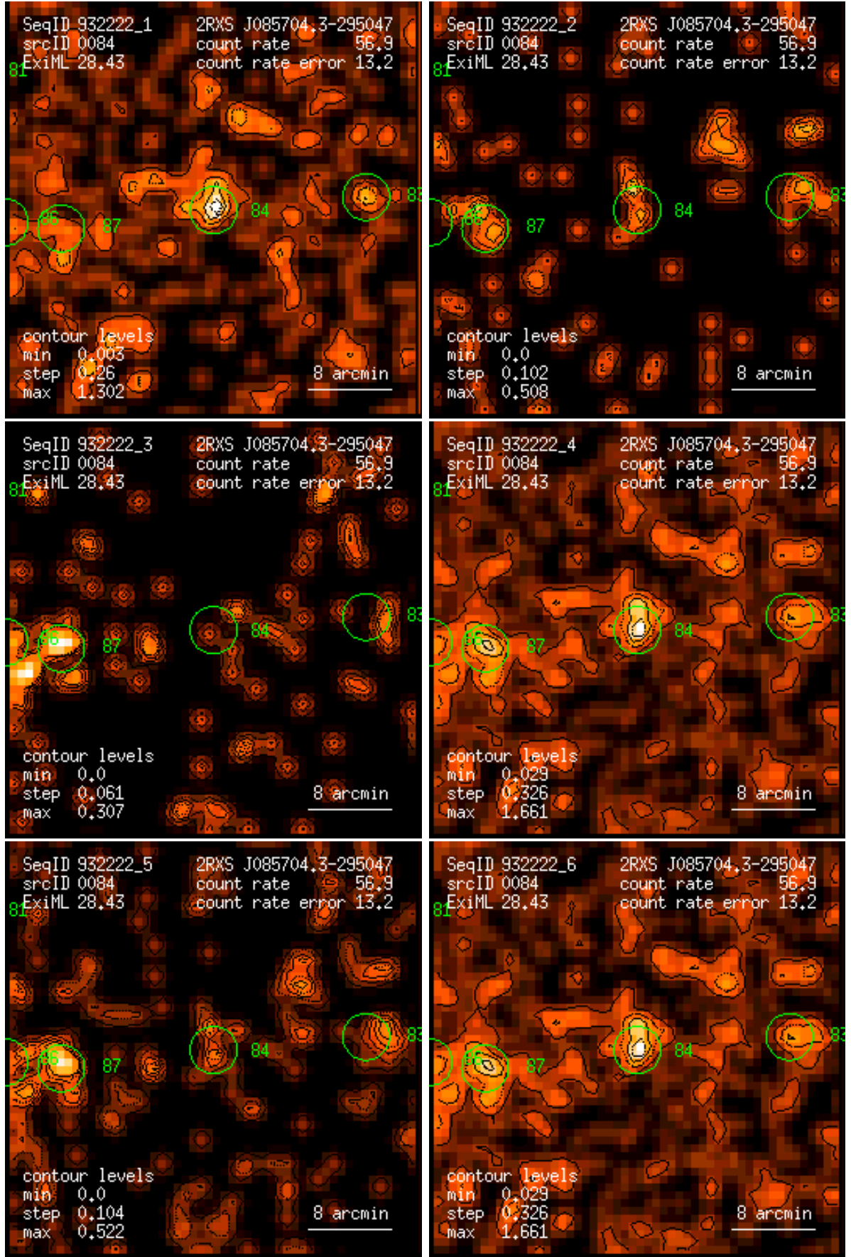
Figure 84: RASS 932222: detection 0084: band rate images, Gaussian filter: (1) PSPC channels 11 – 41, (2) 52 – 90, (3) 91 – 201, (4) 11 – 235, (5) 52 – 201, (6) 11 – 201. Broad band rates in counts/ks. Band rate contour levels in counts/ks/arcmin 2 .
