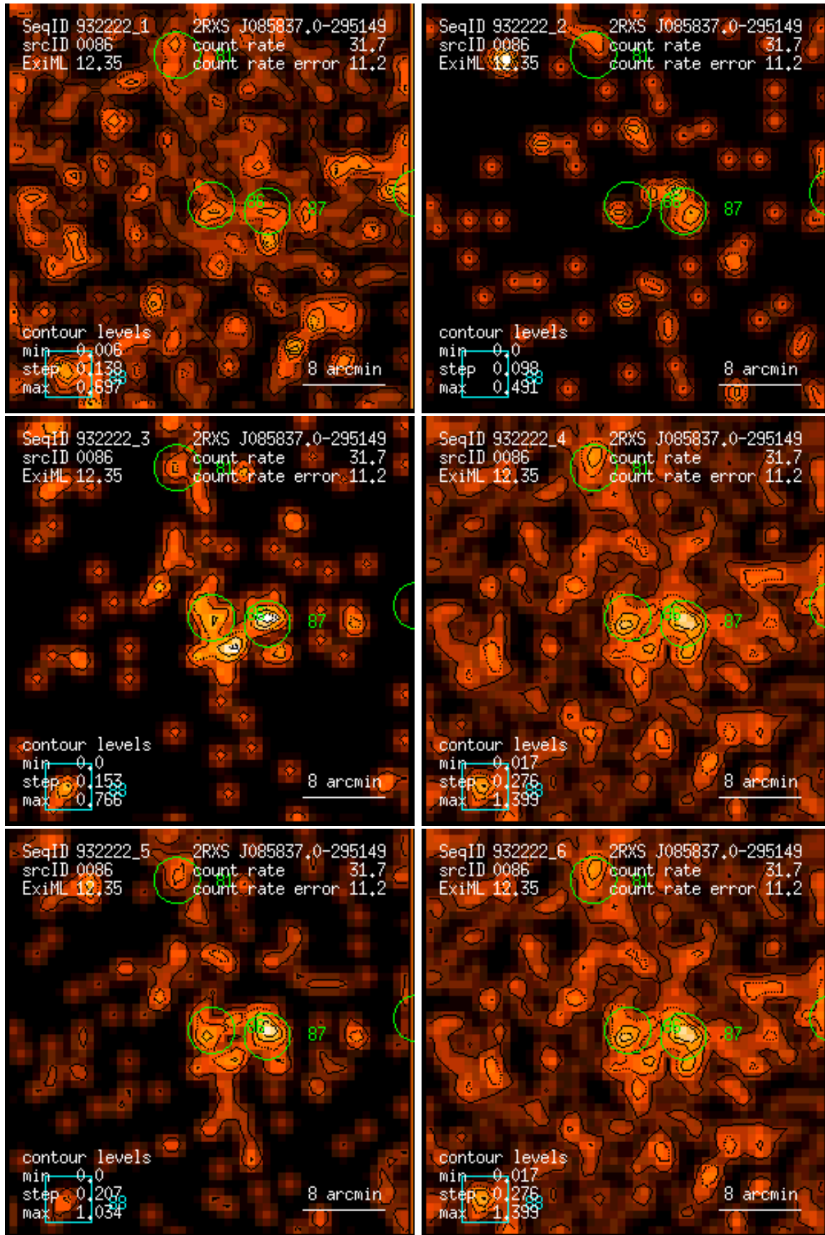
Figure 86: RASS 932222: detection 0086: band rate images, Gaussian filter: (1) PSPC channels 11 – 41, (2) 52 – 90, (3) 91 – 201, (4) 11 – 235, (5) 52 – 201, (6) 11 – 201. Broad band rates in counts/ks. Band rate contour levels in counts/ks/arcmin 2 .
