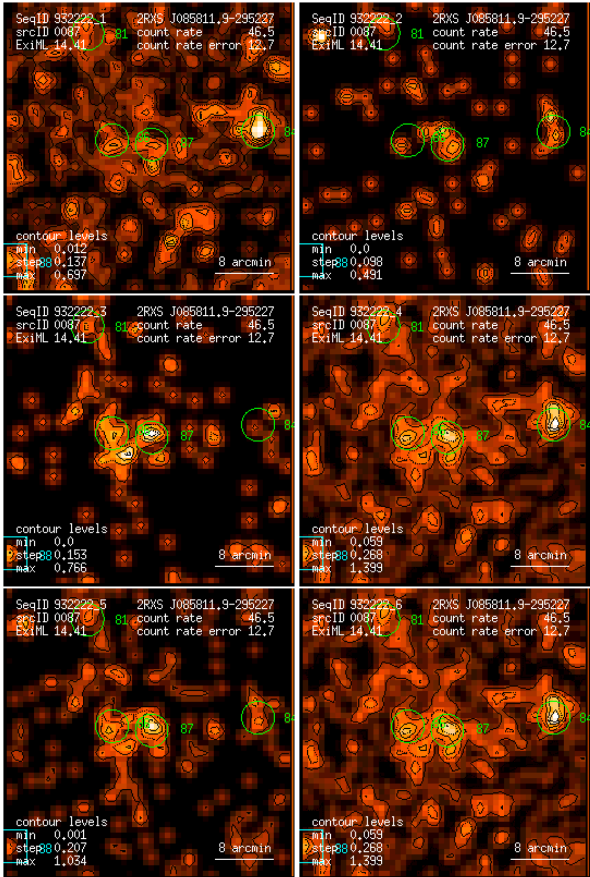
Figure 87: RASS 932222: detection 0087: band rate images, Gaussian filter: (1) PSPC channels 11 – 41, (2) 52 – 90, (3) 91 – 201, (4) 11 – 235, (5) 52 – 201, (6) 11 – 201. Broad band rates in counts/ks. Band rate contour levels in counts/ks/arcmin 2 .
