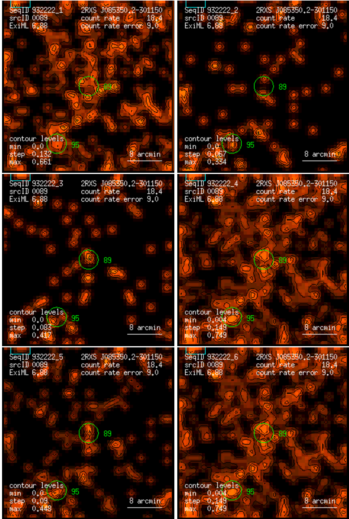
Figure 89: RASS 932222: detection 0089: band rate images, Gaussian filter: (1) PSPC channels 11 – 41, (2) 52 – 90, (3) 91 – 201, (4) 11 – 235, (5) 52 – 201, (6) 11 – 201. Broad band rates in counts/ks. Band rate contour levels in counts/ks/arcmin 2 .
