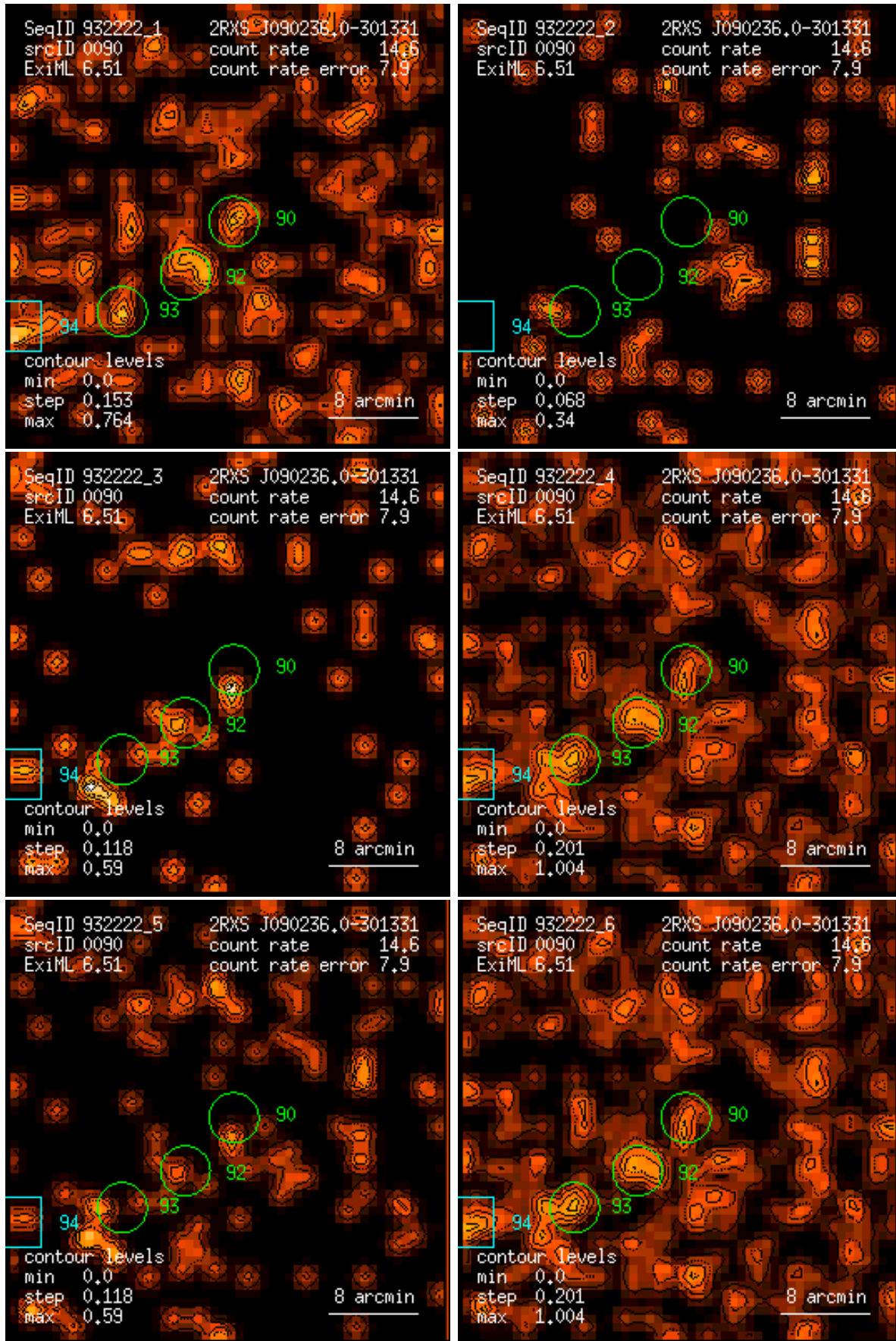
Figure 90: RASS 932222: detection 0090: band rate images, Gaussian filter: (1) PSPC channels 11 – 41, (2) 52 – 90, (3) 91 – 201, (4) 11 – 235, (5) 52 – 201, (6) 11 – 201. Broad band rates in counts/ks. Band rate contour levels in counts/ks/arcmin 2 .
