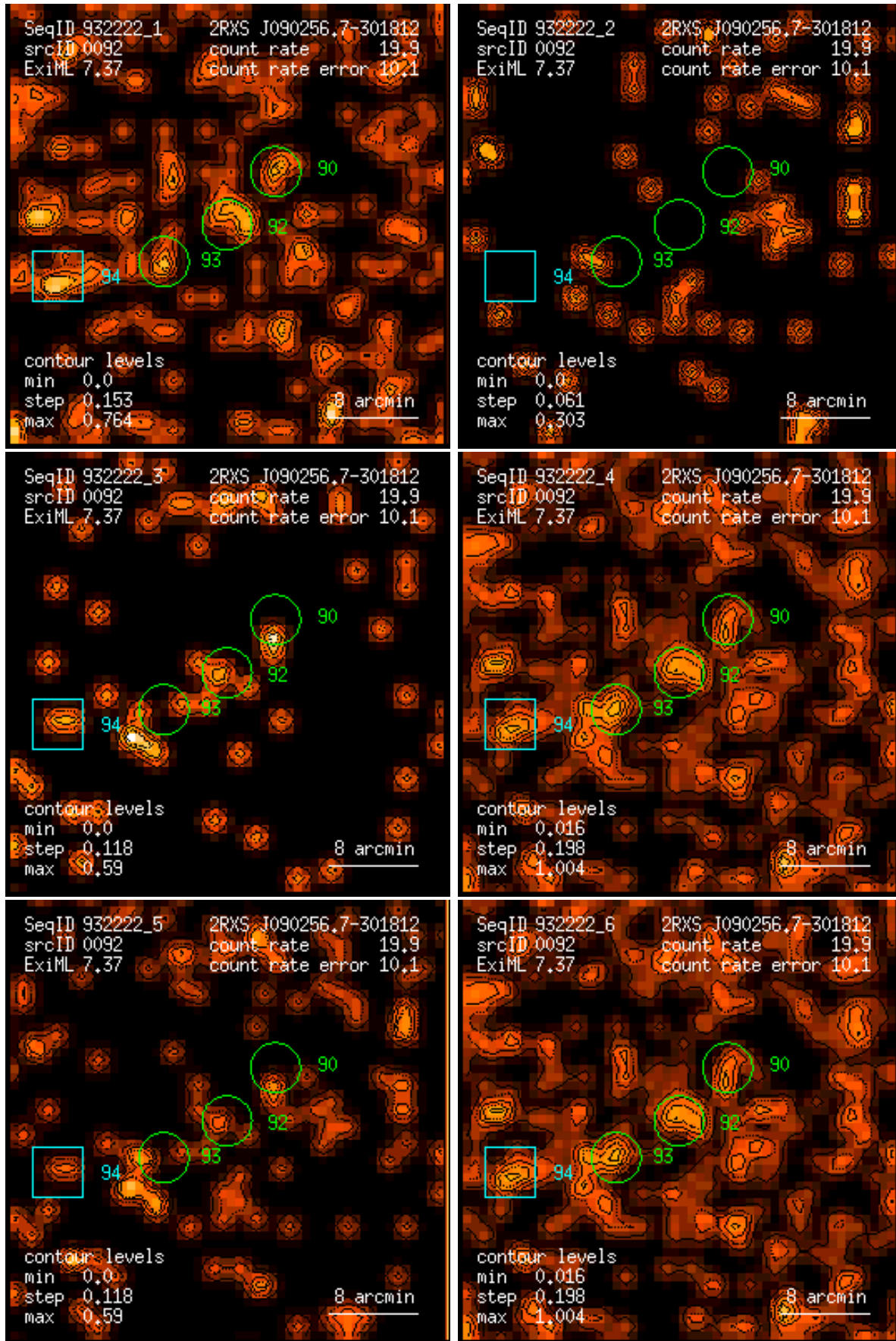
Figure 92: RASS 932222: detection 0092: band rate images, Gaussian filter: (1) PSPC channels 11 – 41, (2) 52 – 90, (3) 91 – 201, (4) 11 – 235, (5) 52 – 201, (6) 11 – 201. Broad band rates in counts/ks. Band rate contour levels in counts/ks/arcmin 2 .
