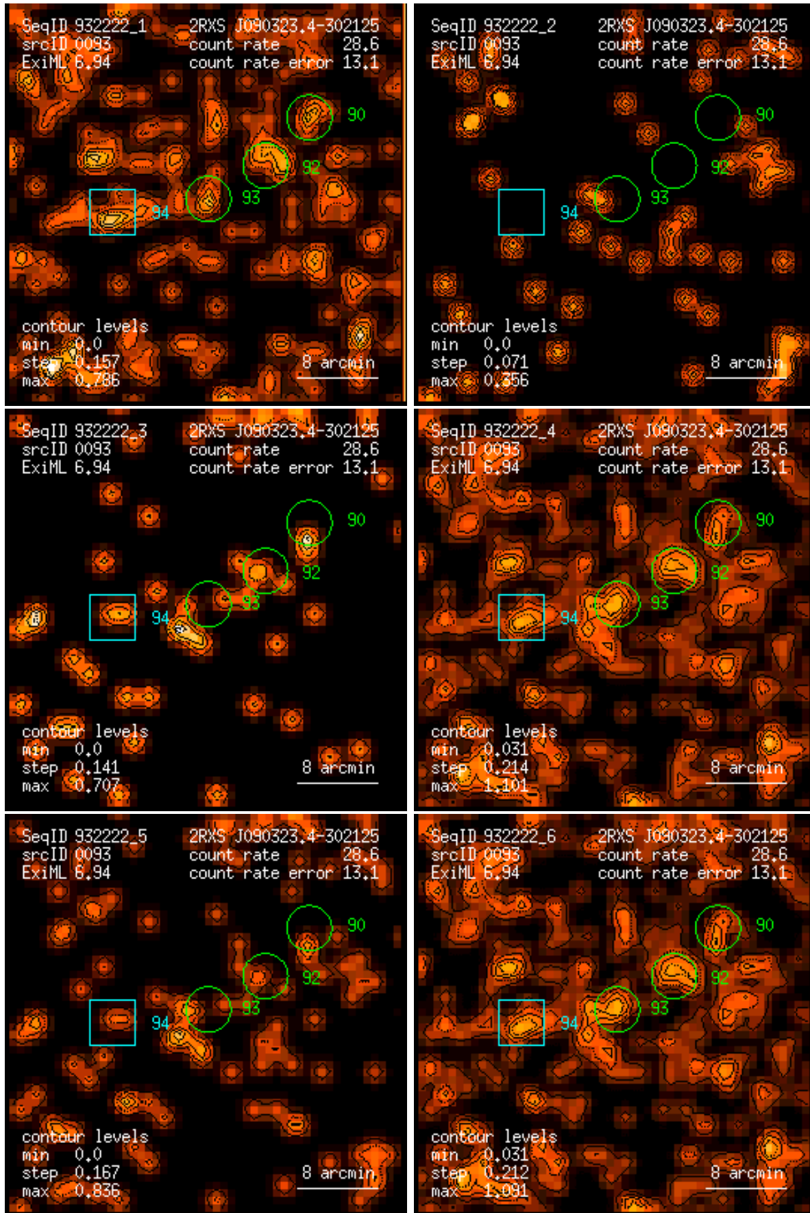
Figure 93: RASS 932222: detection 0093: band rate images, Gaussian filter: (1) PSPC channels 11 – 41, (2) 52 – 90, (3) 91 – 201, (4) 11 – 235, (5) 52 – 201, (6) 11 – 201. Broad band rates in counts/ks. Band rate contour levels in counts/ks/arcmin 2 .
