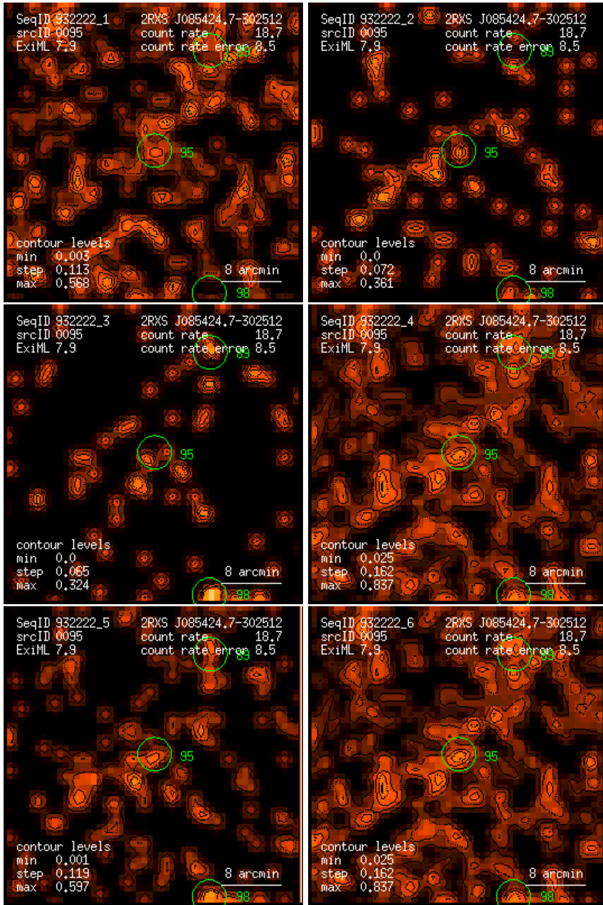
Figure 95: RASS 932222: detection 0095: band rate images, Gaussian filter: (1) PSPC channels 11 – 41, (2) 52 – 90, (3) 91 – 201, (4) 11 – 235, (5) 52 – 201, (6) 11 – 201. Broad band rates in counts/ks. Band rate contour levels in counts/ks/arcmin 2 .
