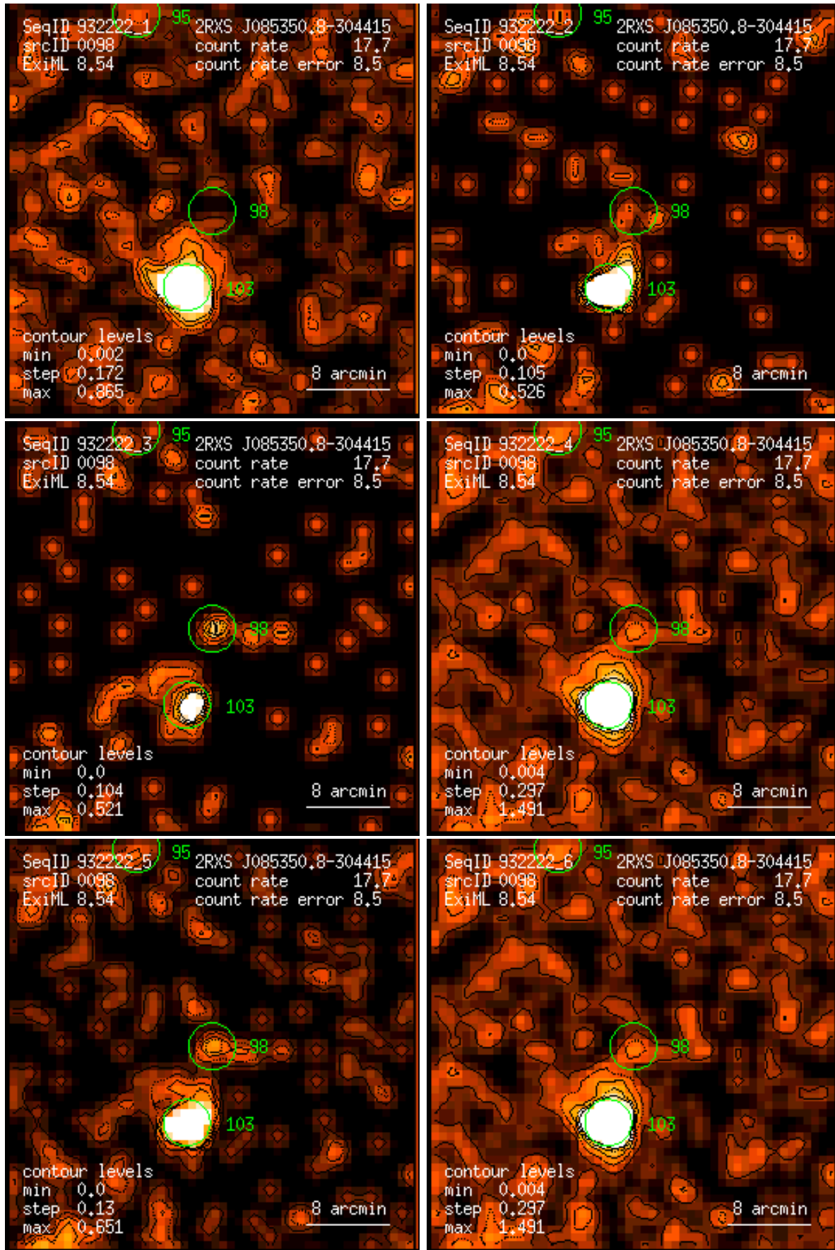
Figure 98: RASS 932222: detection 0098: band rate images, Gaussian filter: (1) PSPC channels 11 – 41, (2) 52 – 90, (3) 91 – 201, (4) 11 – 235, (5) 52 – 201, (6) 11 – 201. Broad band rates in counts/ks. Band rate contour levels in counts/ks/arcmin 2 .
