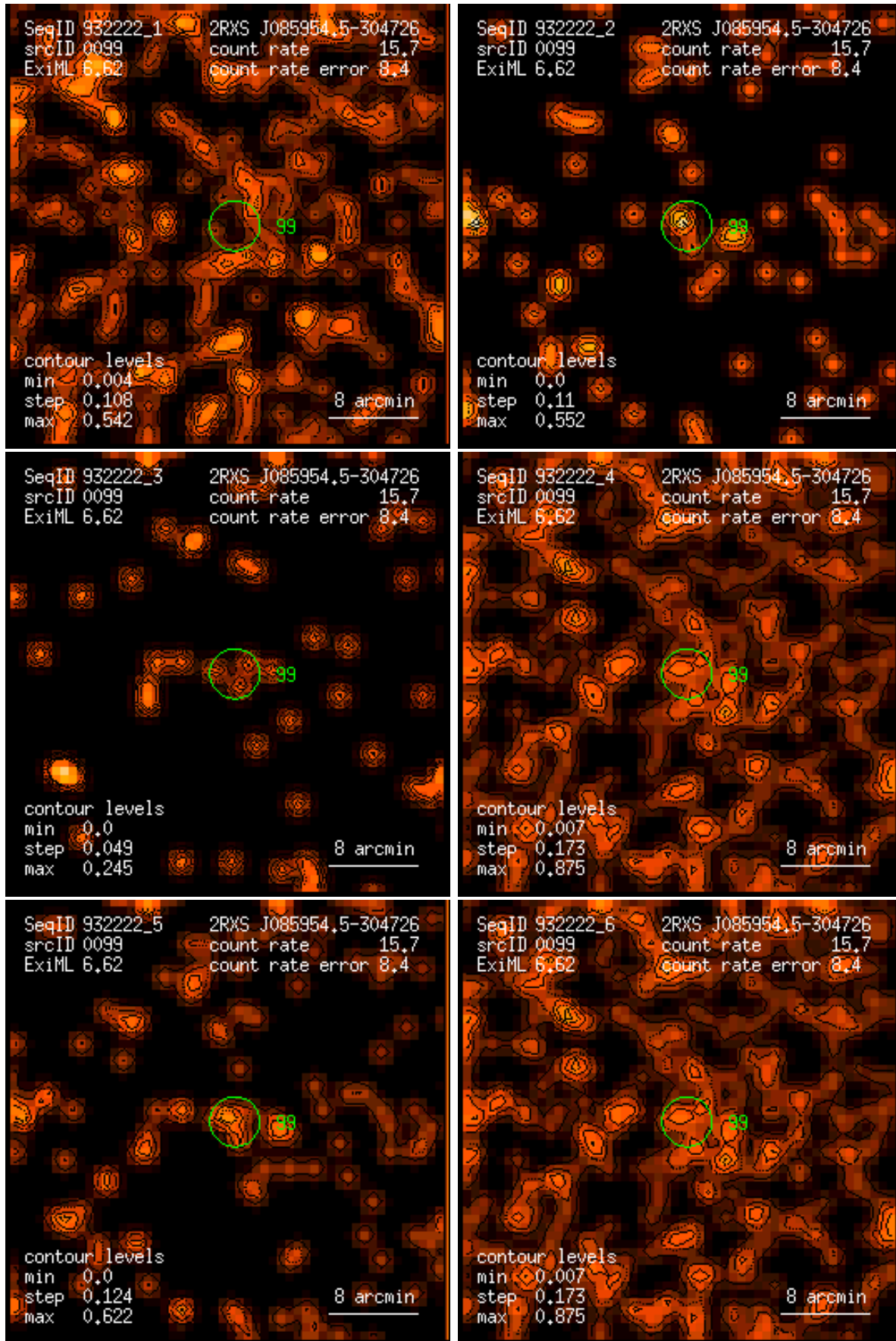
Figure 99: RASS 932222: detection 0099: band rate images, Gaussian filter: (1) PSPC channels 11 – 41, (2) 52 – 90, (3) 91 – 201, (4) 11 – 235, (5) 52 – 201, (6) 11 – 201. Broad band rates in counts/ks. Band rate contour levels in counts/ks/arcmin 2 .
