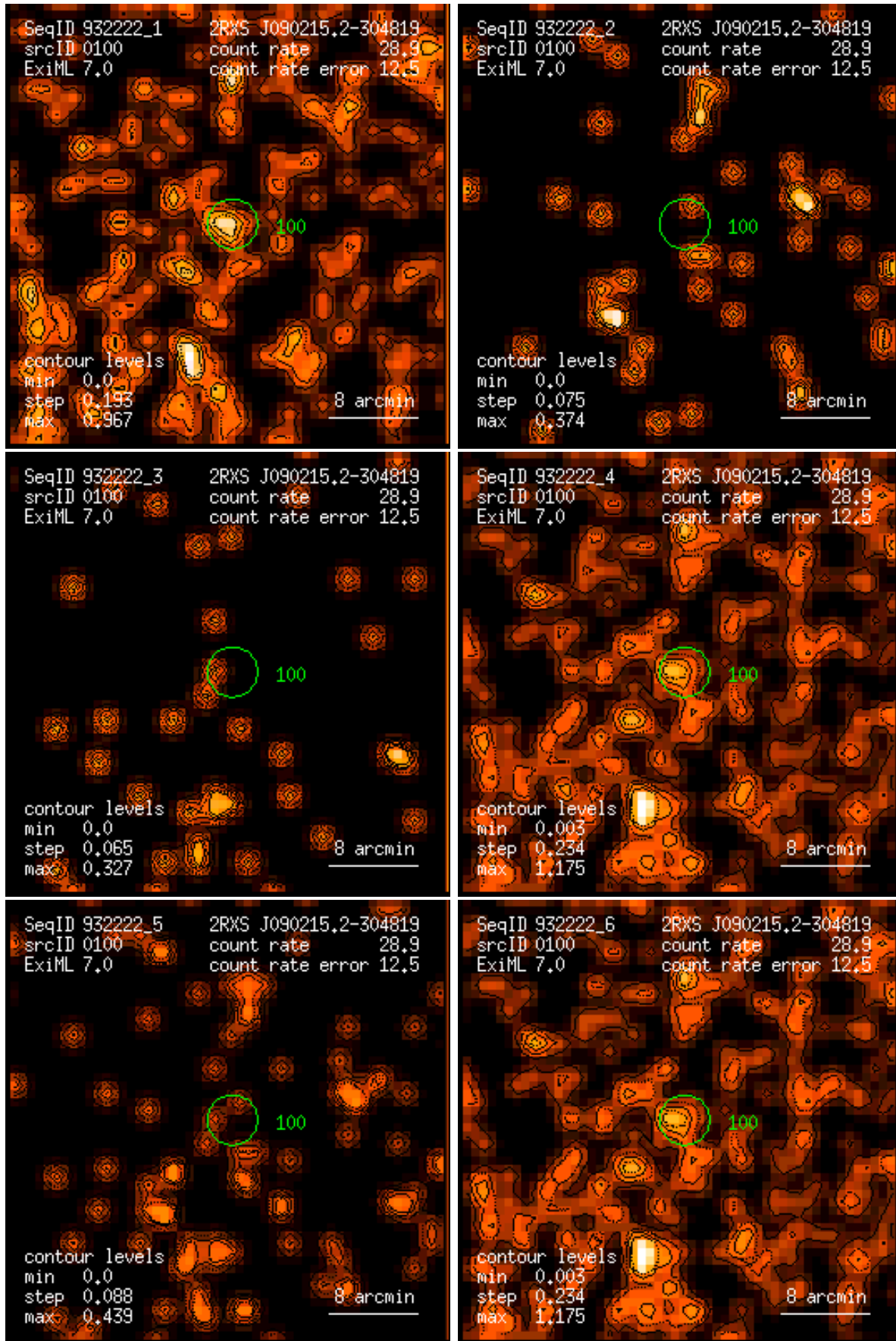
Figure 100: RASS 932222: detection 0100: band rate images, Gaussian filter: (1) PSPC channels 11 – 41, (2) 52 – 90, (3) 91 – 201, (4) 11 – 235, (5) 52 – 201, (6) 11 – 201. Broad band rates in counts/ks. Band rate contour levels in counts/ks/arcmin 2 .
