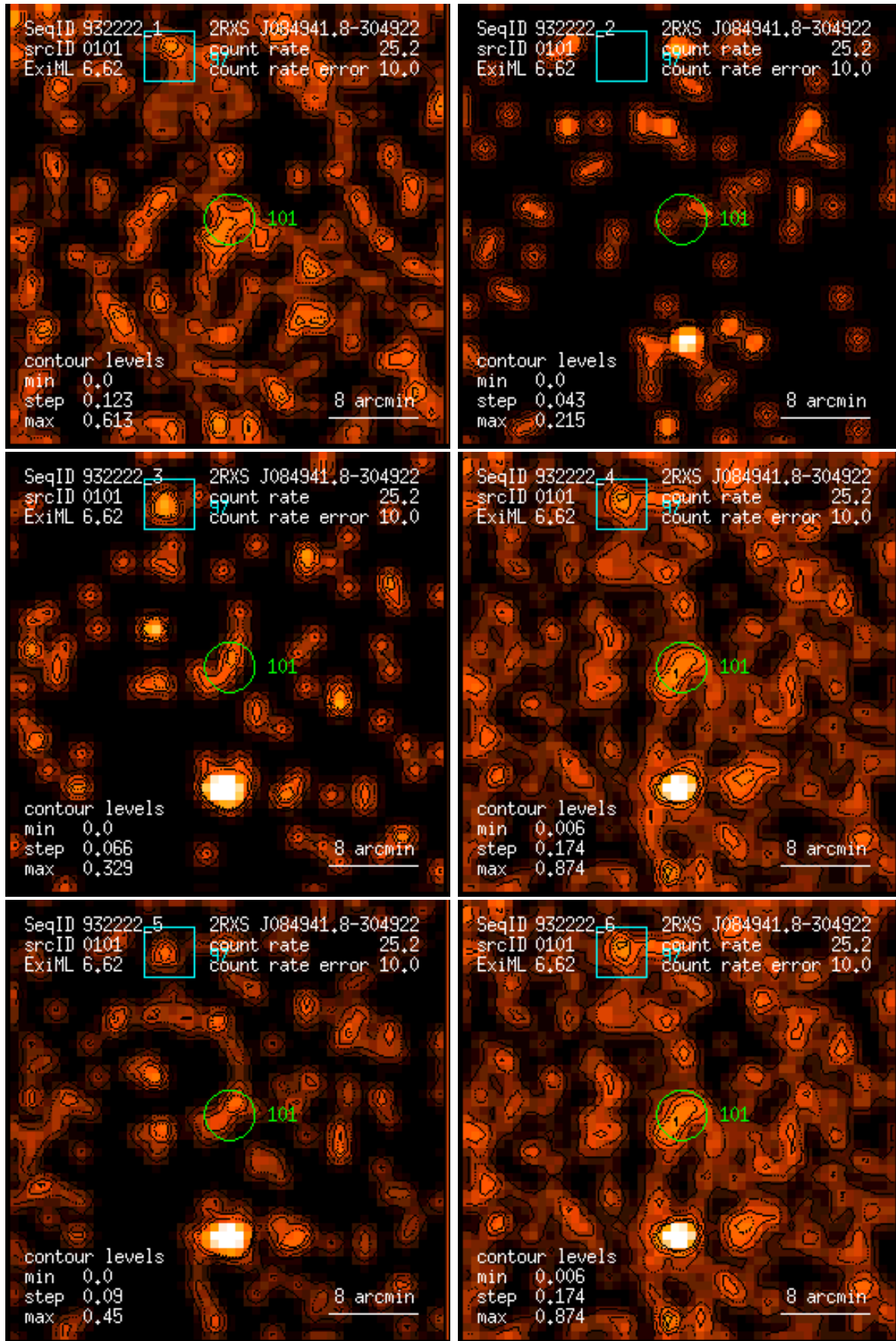
Figure 101: RASS 932222: detection 0101: band rate images, Gaussian filter: (1) PSPC channels 11 – 41, (2) 52 – 90, (3) 91 – 201, (4) 11 – 235, (5) 52 – 201, (6) 11 – 201. Broad band rates in counts/ks. Band rate contour levels in counts/ks/arcmin 2 .
