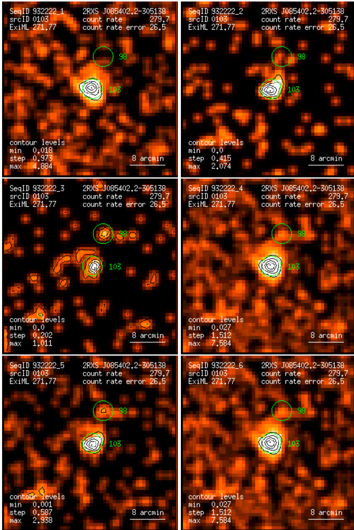
Figure 103: RASS 932222: detection 0103: band rate images, Gaussian filter: (1) PSPC channels 11 – 41, (2) 52 – 90, (3) 91 – 201, (4) 11 – 235, (5) 52 – 201, (6) 11 – 201. Broad band rates in counts/ks. Band rate contour levels in counts/ks/arcmin 2 .
