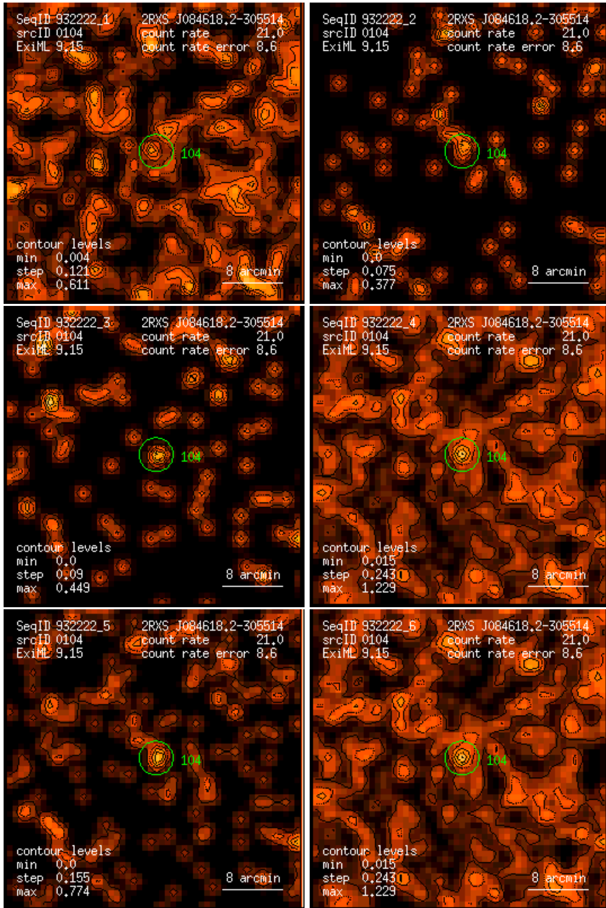
Figure 104: RASS 932222: detection 0104: band rate images, Gaussian filter: (1) PSPC channels 11 – 41, (2) 52 – 90, (3) 91 – 201, (4) 11 – 235, (5) 52 – 201, (6) 11 – 201. Broad band rates in counts/ks. Band rate contour levels in counts/ks/arcmin 2 .
