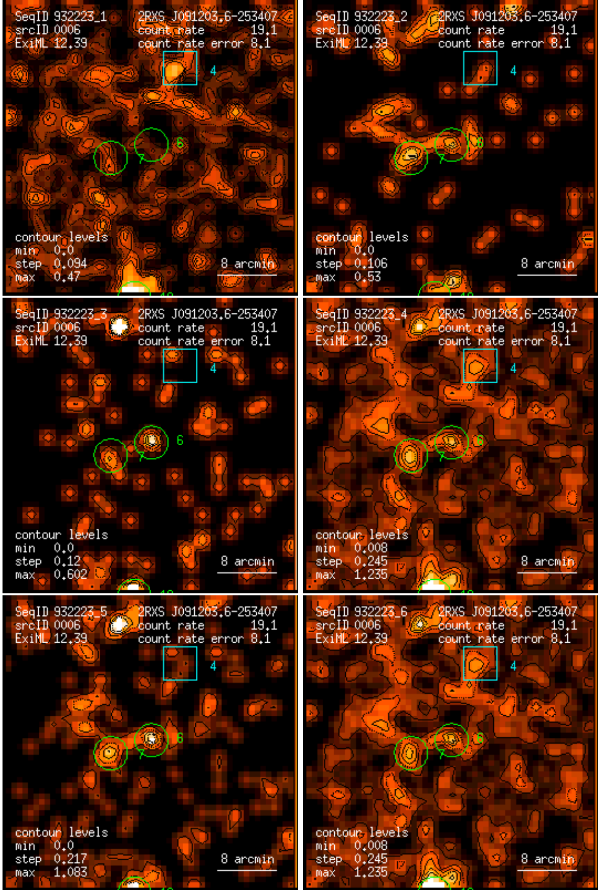
Figure 6: RASS 932223: detection 0006: band rate images, Gaussian filter: (1) PSPC channels 11 – 41, (2) 52 – 90, (3) 91 – 201, (4) 11 – 235, (5) 52 – 201, (6) 11 – 201. Broad band rates in counts/ks. Band rate contour levels in counts/ks/arcmin 2 .
