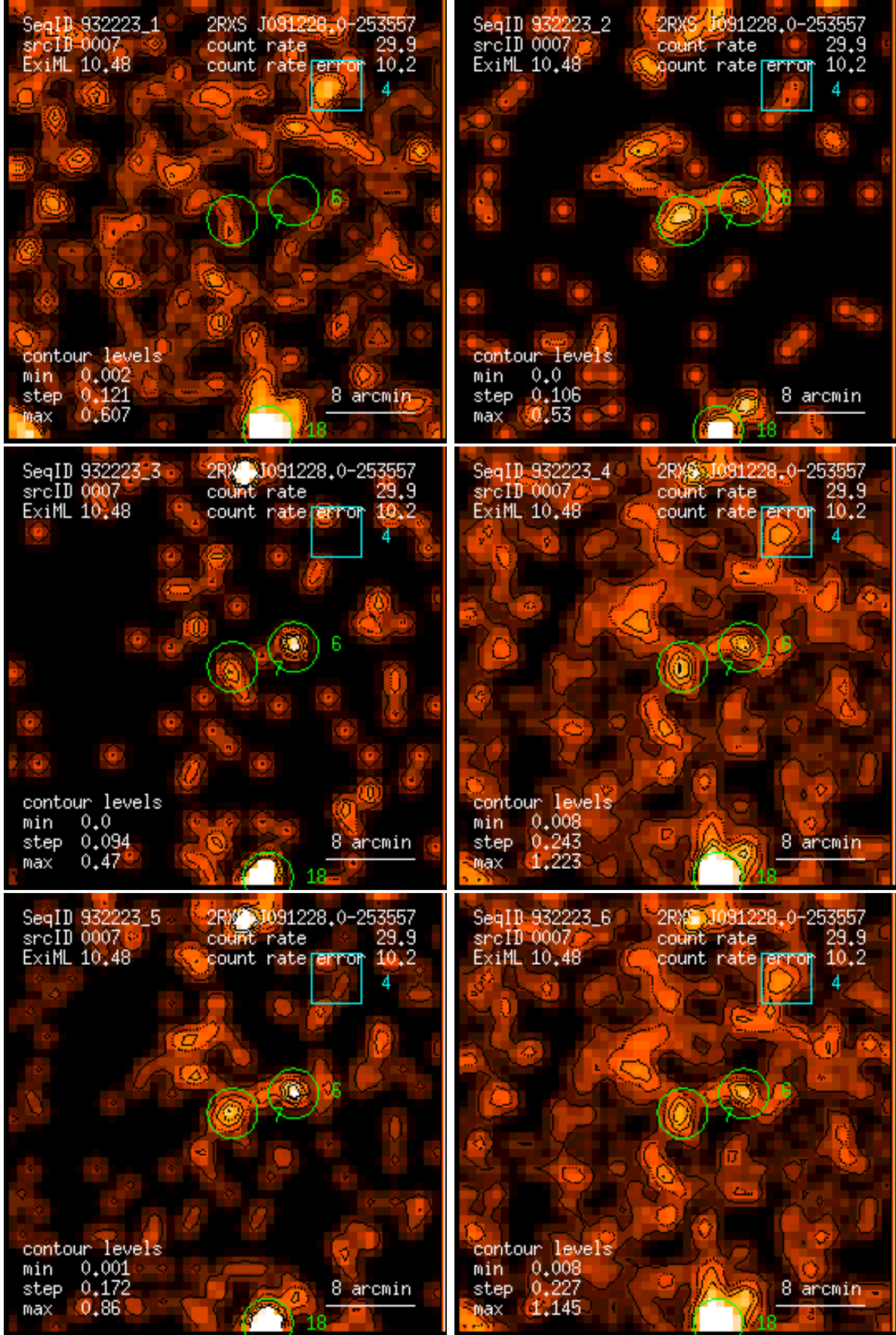
Figure 7: RASS 932223: detection 0007: band rate images, Gaussian filter: (1) PSPC channels 11 – 41, (2) 52 – 90, (3) 91 – 201, (4) 11 – 235, (5) 52 – 201, (6) 11 – 201. Broad band rates in counts/ks. Band rate contour levels in counts/ks/arcmin 2 .
