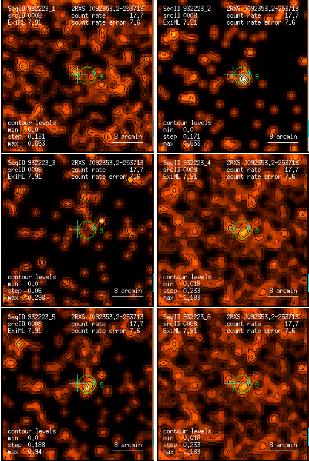
Figure 8: RASS 932223: detection 0008: band rate images, Gaussian filter: (1) PSPC channels 11 – 41, (2) 52 – 90, (3) 91 – 201, (4) 11 – 235, (5) 52 – 201, (6) 11 – 201. Broad band rates in counts/ks. Band rate contour levels in counts/ks/arcmin 2 .
