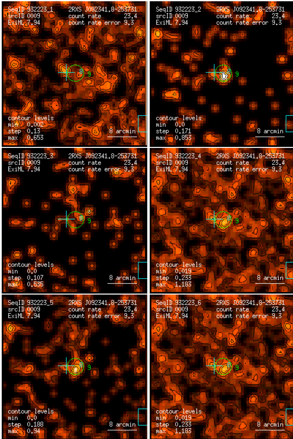
Figure 9: RASS 932223: detection 0009: band rate images, Gaussian filter: (1) PSPC channels 11 – 41, (2) 52 – 90, (3) 91 – 201, (4) 11 – 235, (5) 52 – 201, (6) 11 – 201. Broad band rates in counts/ks. Band rate contour levels in counts/ks/arcmin 2 .
