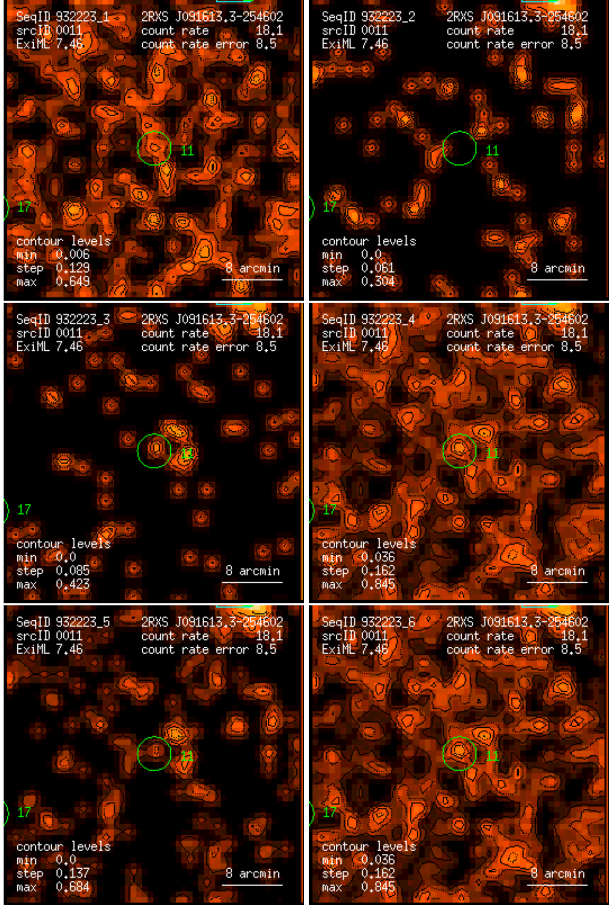
Figure 11: RASS 932223: detection 0011: band rate images, Gaussian filter: (1) PSPC channels 11 – 41, (2) 52 – 90, (3) 91 – 201, (4) 11 – 235, (5) 52 – 201, (6) 11 – 201. Broad band rates in counts/ks. Band rate contour levels in counts/ks/arcmin 2 .
