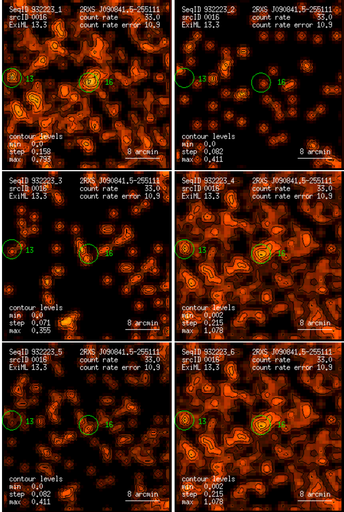
Figure 16: RASS 932223: detection 0016: band rate images, Gaussian filter: (1) PSPC channels 11 – 41, (2) 52 – 90, (3) 91 – 201, (4) 11 – 235, (5) 52 – 201, (6) 11 – 201. Broad band rates in counts/ks. Band rate contour levels in counts/ks/arcmin 2 .
