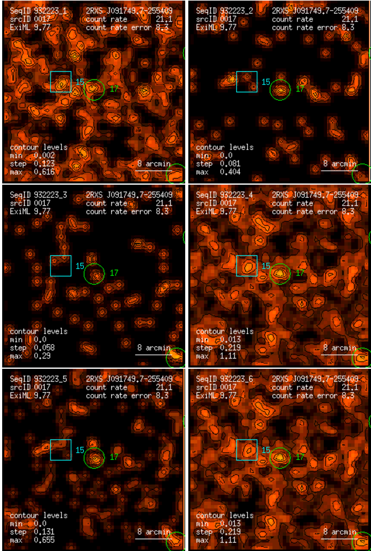
Figure 17: RASS 932223: detection 0017: band rate images, Gaussian filter: (1) PSPC channels 11 – 41, (2) 52 – 90, (3) 91 – 201, (4) 11 – 235, (5) 52 – 201, (6) 11 – 201. Broad band rates in counts/ks. Band rate contour levels in counts/ks/arcmin 2 .
